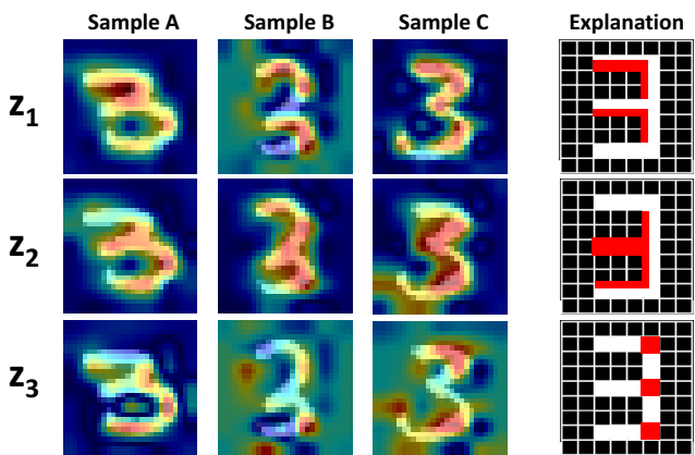
Figure 1. We propose to visually explain variational autoencoders. Each element in the latent vector (here z_1 - z_3 ) can be explained separately with our attention maps, visualizing consistent explanations across different samples.
