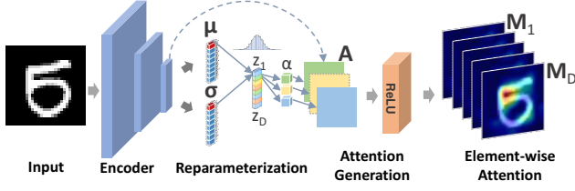
Figure 2. Element-wise attention generation with a VAE.
