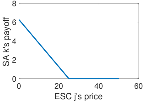
Fig. 2. Variation of SA k 's payoff as a function of \tilde{p}_j for the same example as in Figure 1 ( \Lambda = 300, W = 150, v = 3, q_j = 0.5 ). When \tilde{p}_j > 25 , SA k does not obtain information from the ESC.
