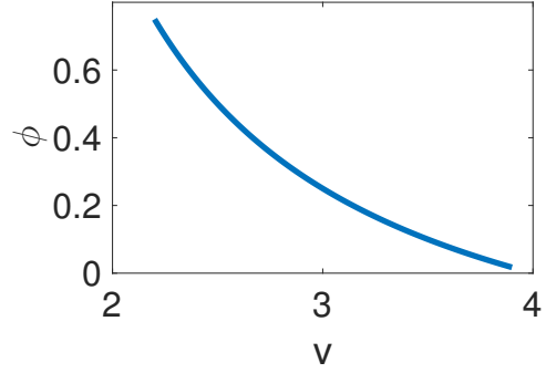
Fig. 1. The variation of \phi as a function of v in an example scenario with \Lambda = 300 , W = 150 , q_j = 0.5 .
