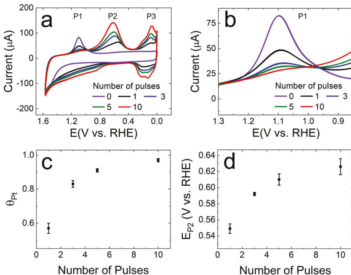
Fig. 2 (a) CVs recorded before and after HT Pt electrodeposition onto Au_{147} DENs using the indicated number of pulses. Peaks P1, P2, and P3 correspond to AuO_x reduction, PtO_x reduction, and Pt-H adsorption/desorption (Pt-hydride) peaks, respectively. (b) Expanded view of Peaks P1, showing that the Au_{147} NP surface is nearly completely covered after 3 to 5 HT pulses. (c) Pt coverage ( \theta_{Pt} ) as a function of pulse number. (d) The position of Peak P2 as a function of pulse number. The electrolyte was N_2 -purged 0.10 M HClO_4 and the scan rate was 100\text{ mV s}^{-1} .
