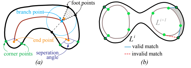
Fig. 4: Corner extraction and matching. (a) illustrates the corner (i.e., green dots) extraction using a simplified medial axis (the dark red curve) of a slice of a twisted U shape. The simplified medial axis consists of one branch point (blue dot) and three end points (orange dots). Foot points of the branch point are shown as black dots. (b) shows the matching of the corners between two adjacent level sets with a splitting bifurcation. The shaded area shows a highly distorted quad.
