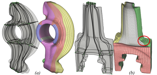
Fig. 13: Results of two CAD models with our method: (a) the rocker arm and (b) the blade. The circle highlights the area with distorted elements in the blade mesh.
