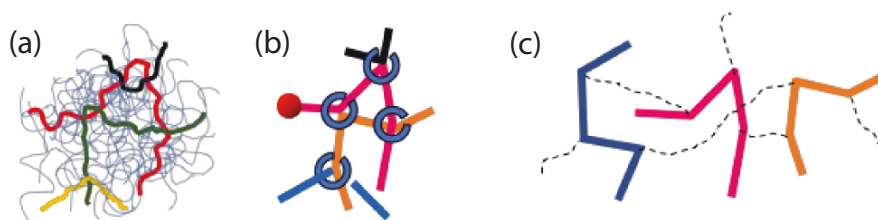
Figure 12. Schematics of slip-spring models. (a) Entangled chains colored in an entangled polymer melt, (b) corresponding slip-spring primitive chain network (PCN) model [178], and (c) a group of chains considered in the Doi and Takimoto (DT) model [179]. Reproduced from [183] with permission from Polymers.
