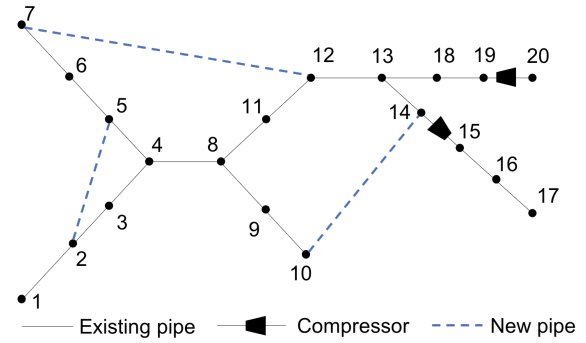
Fig. 2. Modified Belgian natural gas network.
