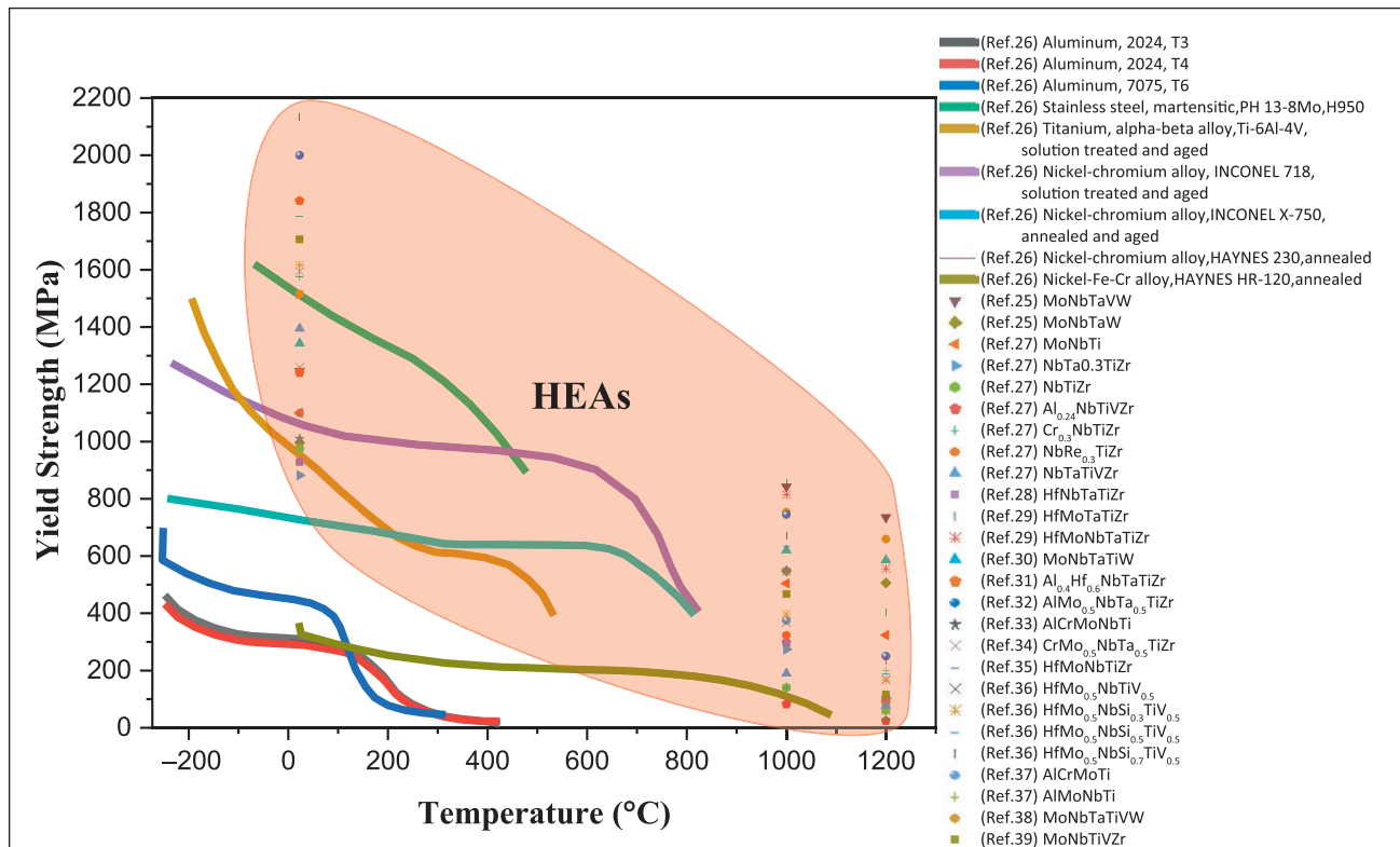
Figure 1. Yield strength ( \sigma_{0.2} ) of several refractory high-entropy alloys 25–39 (HEAs) and conventional stainless steel, aluminum, titanium, and nickel-based alloys. As potential high-temperature materials for structural applications, the HEAs show greater strength. Thermodynamic and mechanical properties for these single-phase and multiphase HEAs are summarized in Reference 40.
