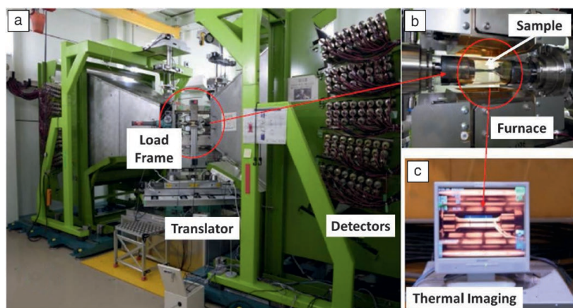
Figure 3. (a) The TAKUMI instrument (Republic of Korea); (b) load frame equipped with a high-temperature chamber; and (c) temperature-mapping monitor. 54
