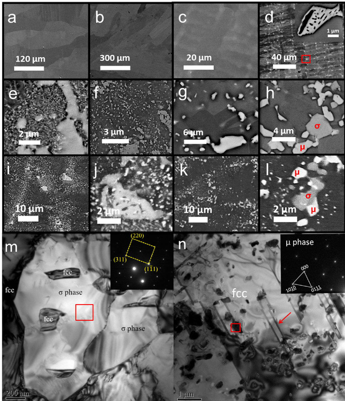
Fig. 8—SEM results of the as-cast CoCrFeNiMo x : (a) x = 0 , (b) x = 0.1 , (c) x = 0.2 , and (d) x = 0.3 ; the 60 pct-rolling Mo 0.3 , annealed at (e) 973 K for 3 ds, (f) 1073 K for 3 ds, (g) 1173 K for 2 ds, (h) 1273 K for 1 days, (i)–(j) 1123 K for 1 h, (k)–(l) 1173 K for 5 h. TEM analyses of Mo 0.3 alloy, (m) the as-cast and (n) 60 pct-rolled, and annealed at 1073 K for 3 ds, from Ref. [79] with permission.
