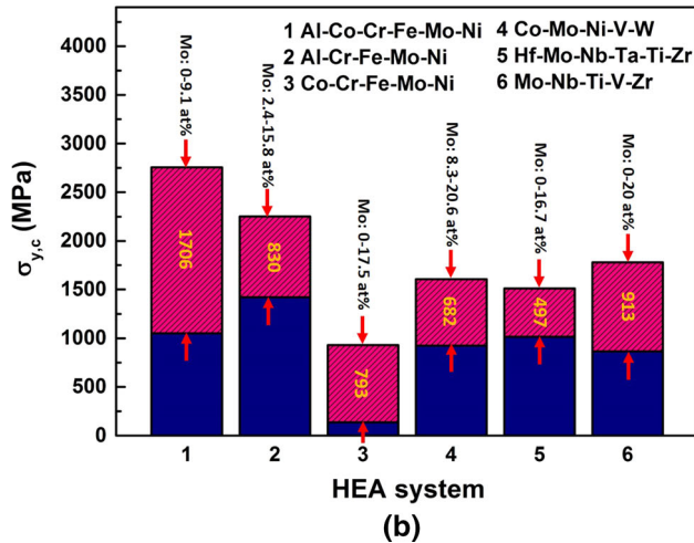
Fig. 7—Values of (a) hardnesses of 3 HEA systems [79–82] and (b) compressive yield strengths of 6 HEA systems [80,81,83–85] with the corresponding Mo-content ranges. The hatched regions are the hardness-change ranges and compressive yield-strength-change ranges of different HEA systems, in (a) and (b), respectively. The colored numbers are the corresponding values of the change ranges (Color figure online).
