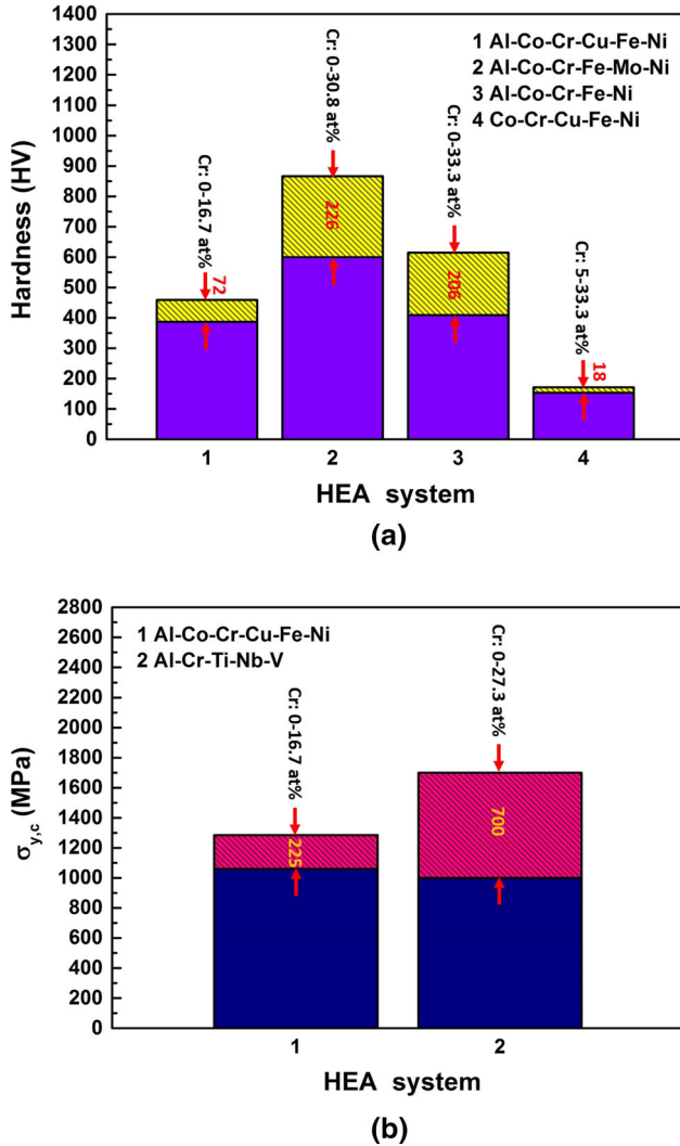
Fig. 4—Values of (a) hardnesses of 4 HEA systems [16,71,72] and (b) compressive yield strengths of 2 HEA systems [73,74] with the corresponding Cr-content ranges. The hatched regions are the hardness-change ranges and compressive yield-strength-change ranges of different HEA systems, in (a) and (b), respectively. The colored numbers are the corresponding values of the change ranges (Color figure online).
