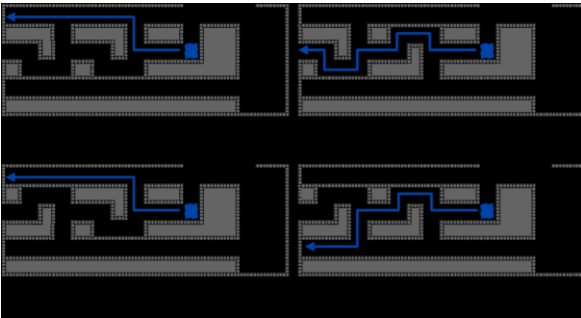
Figure 8: This Figure demonstrates a 2-bit string tunnel. Notice that the tilt sequence hW,N,W,S,W,S,W,N,W_i would only allow a shape to completely traverse bit string tunnel 01.
