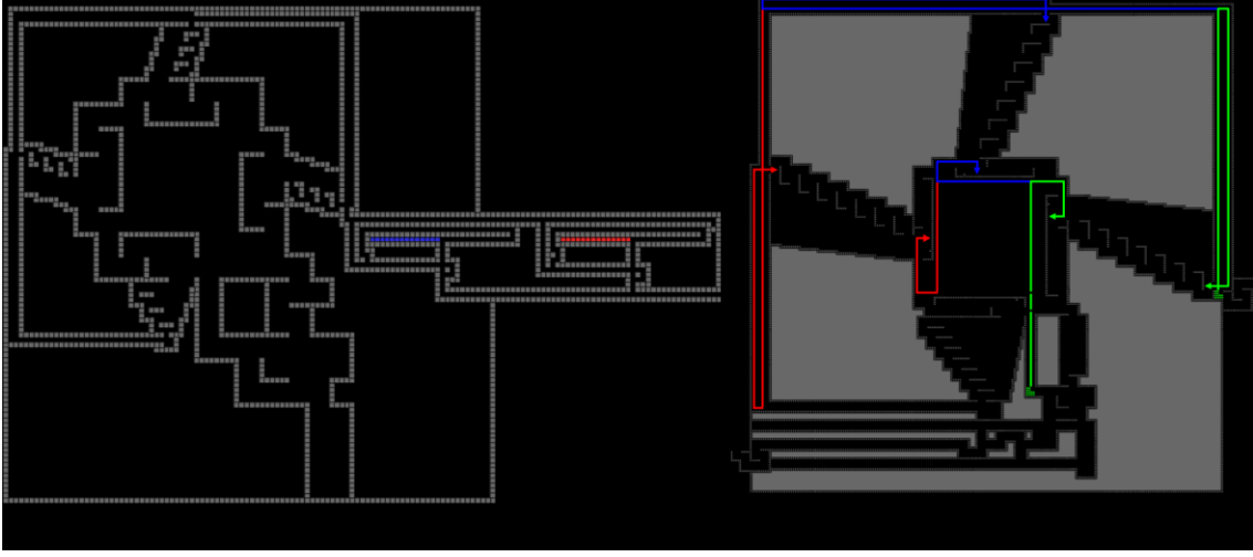
Figure 5: (a) The universal drop-shape constructor from [3] which builds any shape in D_1 . (b) The D_i constructor gadget which allows the dropping of large polyominoes, it also depicts the sequence for selecting a direction to drop from. The paths from D_i constructor gadget look the same in the D_1 .
