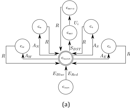
Figure 7: (a) A flowchart where each state represents a set of configurations and the symbols represent sequences that can move from one state to another. The sequences for each of the symbols is shown in Table 4. The sequence marked as U_i is a unique combination of T_0 and T_1 tilt sequences for each i th constructor. Note that after performing the S_{BST}, U_i, R sequences one has successfully relocated the shape located in D_i to D_{i+1} and can add both shapes located in constructor D_{i+1} with either of the A_N, A_E, A_S, A_W sequences. (b) This is an overview of the different sections of the hierarchy constructor. Section 1 is the D_1 shape constructor as shown in [3], section 2 is the bit string tunnels, section 3 is the reset gadget and section 4 is vertices, and allows the target edge to be flipped? This is a one-player unbounded game. The problem is still PSPACE-complete when the edge weights are all strength 1 or 2, and vertices have max degree 3. We address the following equivalent problem.
