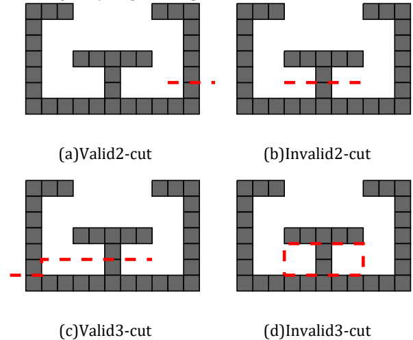
Figure 2: Examples of valid and invalid cuts for a given polyomino. It is important to note that along with direct collision, we consider a cut to be invalid if the resulting
