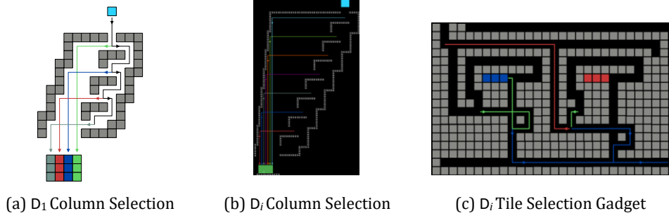
Figure 6: (a) The column selection gadget for D 1 shapes. Assuming the shape to build is at a fixed location, this gadget allows any column to be selected to drop the new tile onto. The number of columns to drop from in this gadget determines the size of the shape we can build. Thus, this is for a drop shape within a 4 \times 4 bounding box. This gadget is repeated on each of the four sides of the drop-shape constructor (with a slightly modified one on the south side in order to allow a non-conflicting move sequence.). (b) The column selection gadget for a 4 \times 4 D i constructor. Notice that the tunnels are large enough to accommodate shapes that fit in a 4 \times 4 bounding box, and the attachment area is twice as big as the D 1 version. This is to allow large polyominoes to be dropped onto any row/column of another large polyomino. (c) The fuel selection gadget for D 1 . Each tile is pulled out with the sequence hE,N,W,S,E,S_i , and stops at the first square. Then the left tile type (blue) is either pulled out of the gadget or put back in the storage area. This shows it being added back to the storage with hE,S,W,N,W,S_i . This sequence puts the next tile type (red) in a decision location. The red tile is selected with the sequence hW,N,W,S,W,S_i . Once the desired shape has been built, one can remove the remaining fuel tiles off the board with hE,N,W,S,E,S,W,S,E,S,W,S,E,W_i . This sequence extracts both tile types off the storage area, and then removes them off the board.
