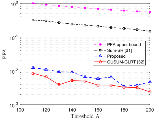
FIGURE 7. Probability of false alarm v.s. threshold.
