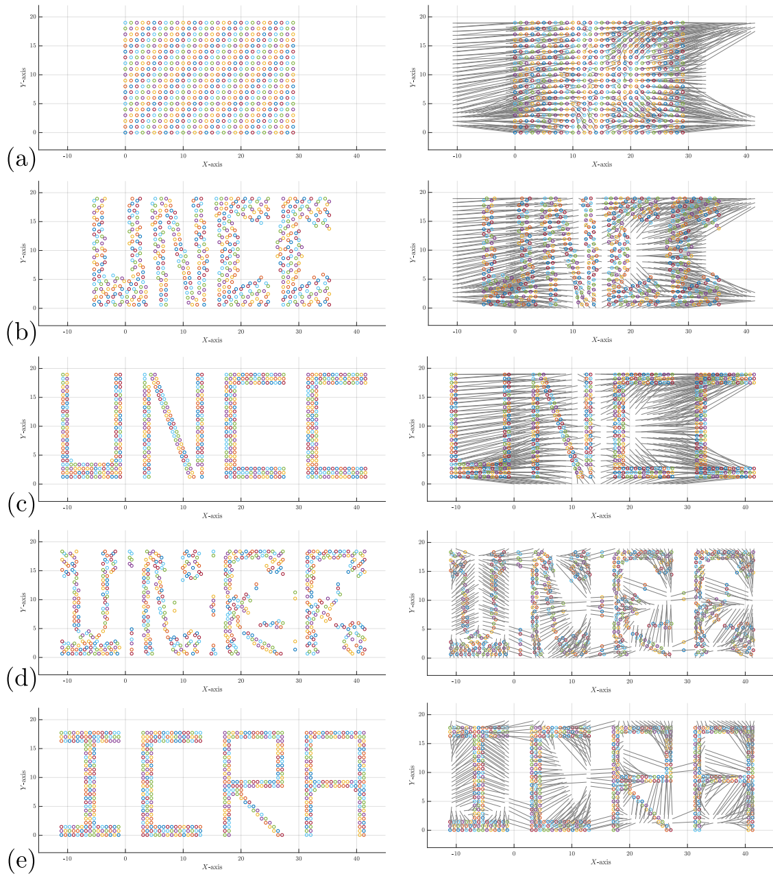
Fig. 5. Simulation of 600 robots moving from an initial formation to two successive goal formations for an assignment problem with variable scale and translation. The left column shows the formations, while the right column additionally shows the robot paths to the next formation for the computed assignments. (a) Initial formation of the robots in a rectangular grid. (b) Intermediate snapshot of the robots moving towards the UNCC goal formation. (c) The robots at the UNCC goal formation. (d) Intermediate snapshot of the robots moving towards the second goal formation of ICRA. (e) The robots at the ICRA goal formation.
