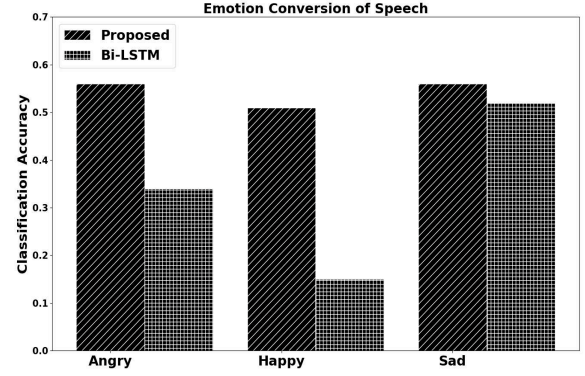
Figure 3: Comparison of emotion classification accuracy.
