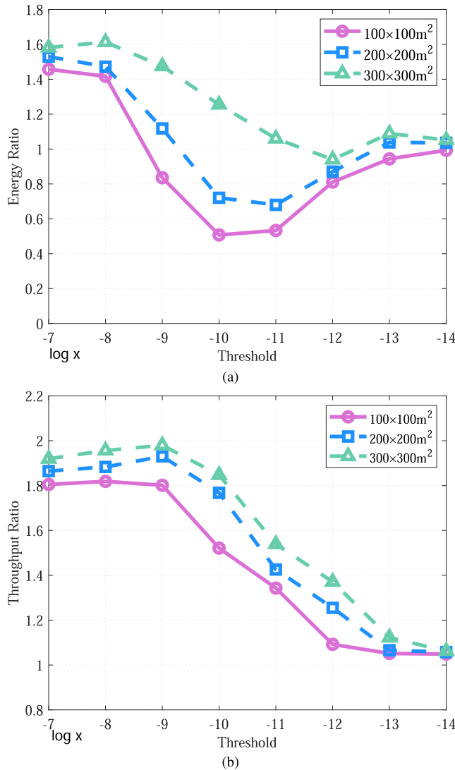
FIGURE 12. Energy Ratio and Throughput Ratio under different BS distribution. (a) Energy Ratio. (b) Throughput Ratio.
