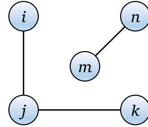
FIGURE 7. Contention graph.
