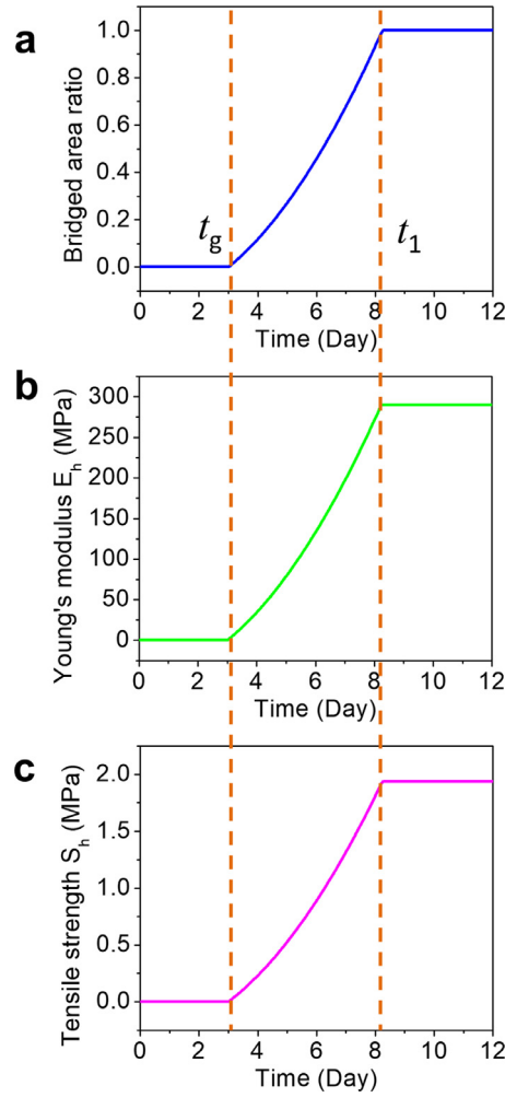
Fig. 11. Theoretically calculated (a) bridged area ratio, (b) effective Young's modulus and (c) effective tensile strength of the cohesive zone in functions of healing days.
