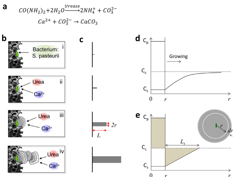
Fig. 5. Model system for the growth of a pillar. (a) Chemical reactions for the production of solute \text{CaCO}_3 . (b) Schematics to show bacteria-assisted nucleation and growth of \text{CaCO}_3 crystals on a ceramic surface. (c) Simplified pillar model for the crystal. (d) The diffusion-controlled growth of a precipitated crystal particle. C_p is the concentration of the solute in the precipitate. C_c is the concentration of the solute in the solution. C_s is the concentration of the solution after precipitation. (e) Simplification of the concentration profile.
