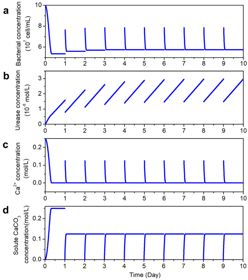
Fig. 9. Evolution of chemical concentrations over 10 days: (a) bacteria, (b) urease, (c) \text{Ca}^{2+} , and (d) solute \text{CaCO}_3 .
