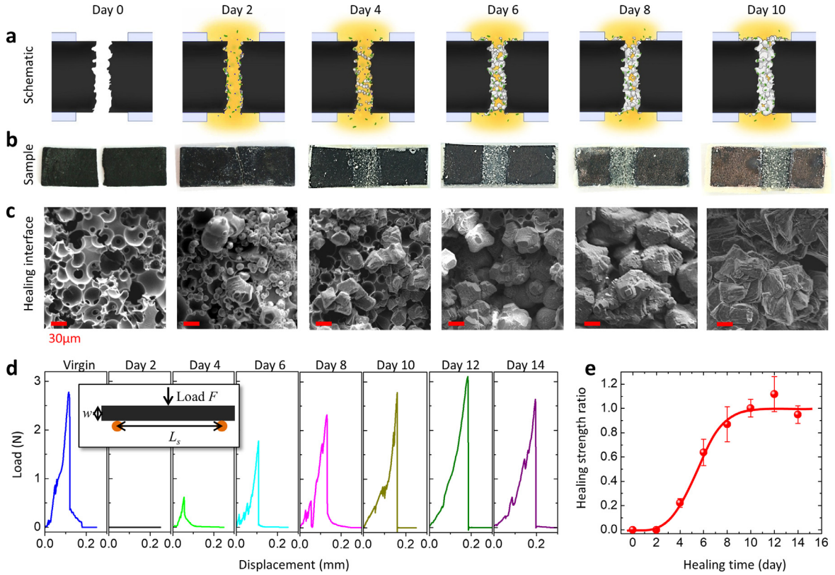
Fig. 3. Experiments of bacteria-assisted healing of ceramics. (a) Schematics of nucleation and growth of bacteria-assisted precipitation of \text{CaCO}_3 crystals on the fracture interface over 10 days. (b) Healing of ceramic plate samples (length 17 mm, width 5.68 mm, and thickness 1.42 mm) over 10 days. (c) SEM images of healing interfaces of ceramic plate samples over 10 days. (d) Load-displacement curves of virgin and healed samples over 10 days in 3PB tests. The inset shows the schematic for the 3PB test, where F is applied load, L_s is span between two supporting points, and w is sample thickness. (e) Healing strength ratios of ceramic plates as a function of healing time. Healing strength ratio is defined as the effective flexural strength of healed samples normalized by that of the virgin sample.
