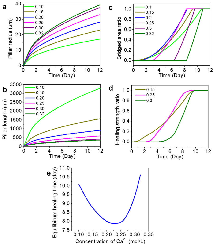
Fig. 15. Effect of the initial \text{Ca}^{2+} concentration. (a) The pillar radii and (b) length for various initial \text{Ca}^{2+} concentrations in functions of time. (c) The bridged area ratios and (d) The healing strength ratios for various initial \text{Ca}^{2+} concentrations in functions of time. (e) The equilibrium healing time in a function of the initial \text{Ca}^{2+} concentration.
