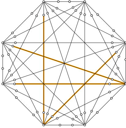
Fig. 4: A drawing of K(8,2) , the complete graph K_8 where every edge is subdivided twice, so that every pair of shortest paths meets at most four times. Two shortest paths that meet four times are shown bold and orange.
