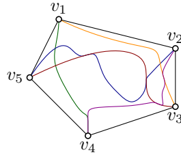
Fig. 1: A drawing of the geodetic graph K_5 that is not philogeodetic. Amongst others, the drawing has a crossing formed by edges v_1v_3 and v_2v_5 . In addition, edges v_1v_4 and v_2v_4 meet but not cross since their meet includes vertex v_4 . Finally, edges v_2v_5 and v_3v_5 meet twice violating the property of philogeodetic drawings.
