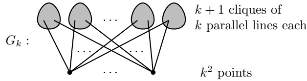
Fig. 5: Structure of the graph G_k .
