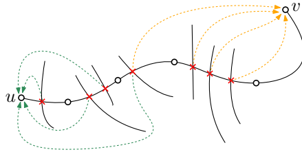
Fig. 2: Every crossing is charged to at least one endpoint of each of the two involved (independent) edges. Vertices are shown as white disks, crossings as red crosses, and charges by dotted arrows. The figure shows an edge uv that is subdivided four times, splitting it into a path with five segments. A crossing along any such segment is assigned to the closest of u or v . For the central segment, both u and v are at the same distance, and any crossing there is assigned to both u and v .
