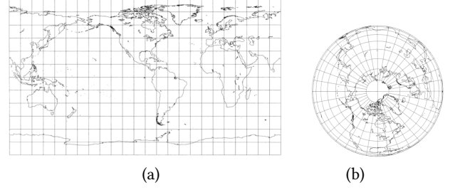
Figure 4: Visualizing Earth with (a) an equirectangular projection where distortion of shapes and areas clearly increase near the poles; and (b) an orthographic projection based on shooting rays from infinity above the north pole [44].
