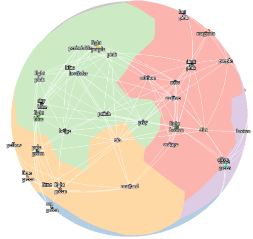
Figure 10: The colors graph obtained by spherical MDS.
