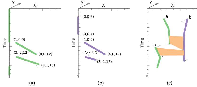
Fig. 4. An event-based dynamic graph in the space-time cube. (a) Position attribute for a node v . Piecewise linear functions encode node position across time. (b) The appearance attribute. Node v only appears over some intervals of time. (c) Edges connect node trajectories as encoded by the edge appearance attribute. The edge traces one or more ruled surfaces in the space-time cube.
