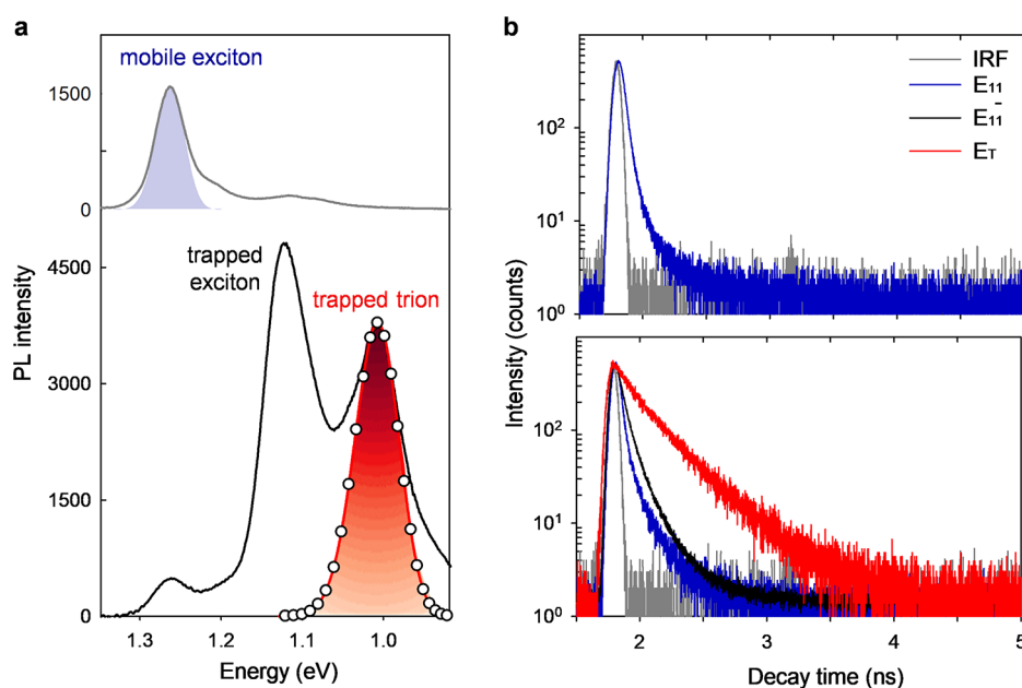
Figure 3. Ultrabright PL of defect-trapped trions. (a) PL spectra of (top) unfunctionalized (6,5)-SWCNTs and (bottom) (6,5)-SWCNT-C 6 H 13 . The excitation wavelength is 565 nm. (b) The PL decays of E_{11} from (top) (6,5)-SWCNTs and (bottom) E_T , E_{11} , and E_{11}^- of (6,5)-SWCNT-C 6 H 13 at room temperature. Note that the instrument response function (IRF) is also plotted.
