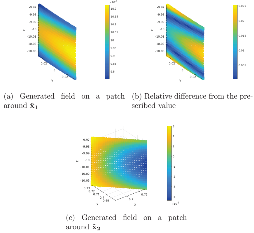
Figure 12: Results of the far field pattern directional control
