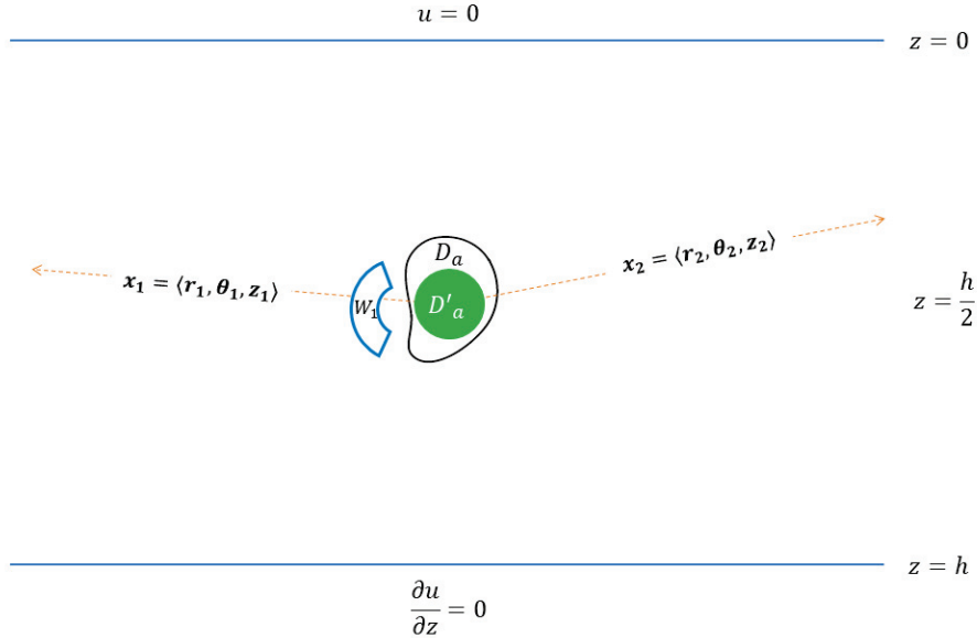
Figure 8: A 3D sketch of the problem geometry for the homogeneous ocean showing the near control and two far field directions \mathbf{x}_1 and \mathbf{x}_2
