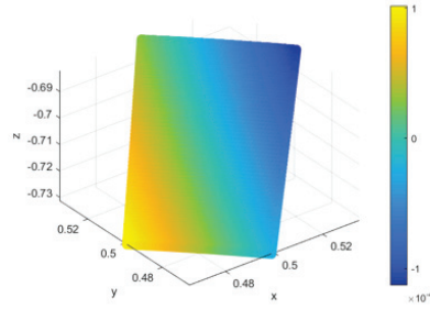
(c) Generated field on a patch around \hat{\mathbf{x}}_2
