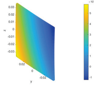
(a) Generated field on a patch around \hat{\mathbf{x}}_1
