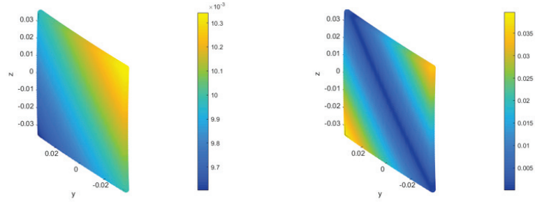
(a) Generated field on a patch around \hat{\mathbf{x}}_1 (b) Relative difference from the prescribed value
