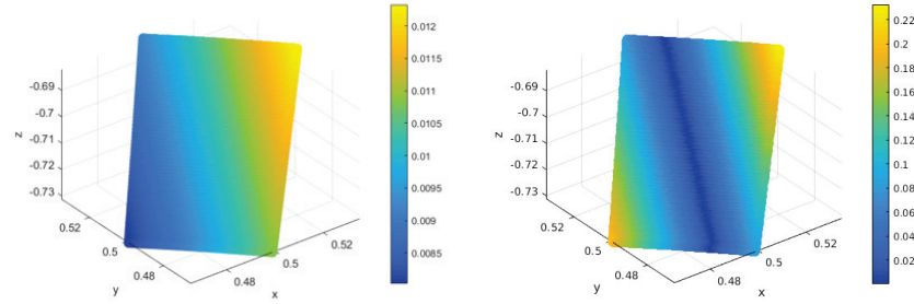
(b) Generated field on a patch around \hat{\mathbf{x}}_2 (c) Relative difference from the prescribed value
