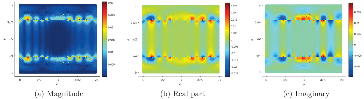
Figure 21: The computed normal velocity on the actual source
