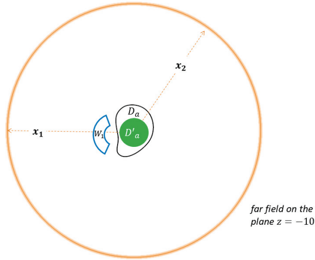
Figure 9: A cross section of the simulation geometry
