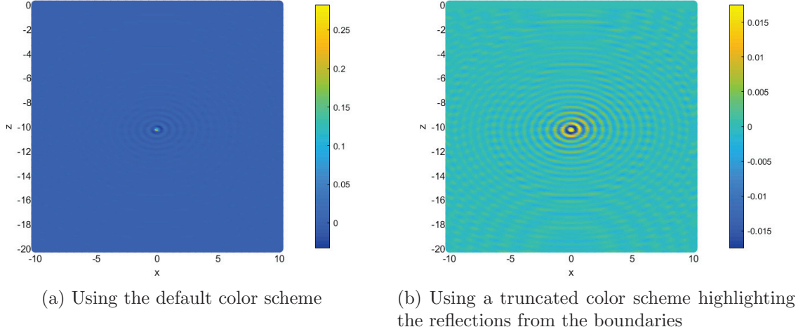
Figure 10: Real part of the generated field on the vertical cross section y = 0
