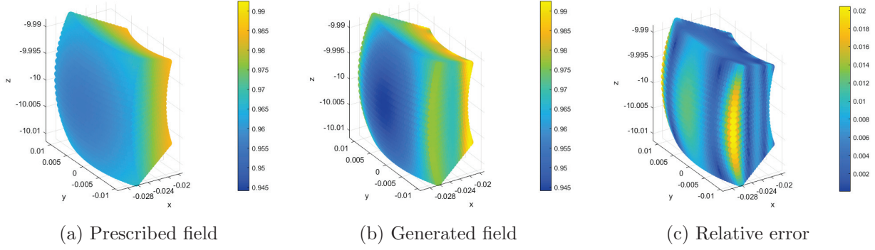
Figure 14: Results of the field synthesis on the near control
