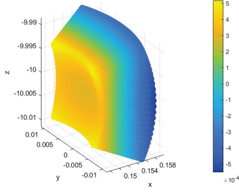
Figure 19: Real part of the generated near field on W_2
