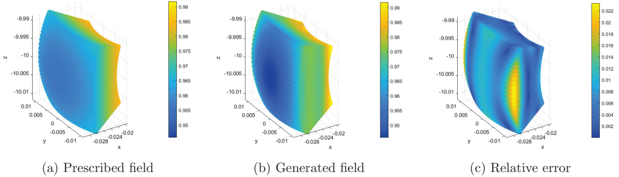
Figure 18: Results of the field synthesis on W_1
