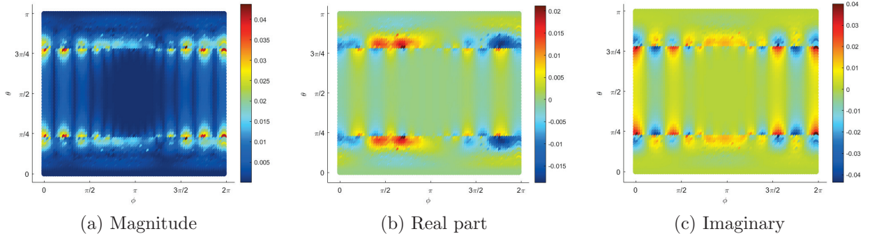
Figure 16: The computed normal velocity on the actual source
