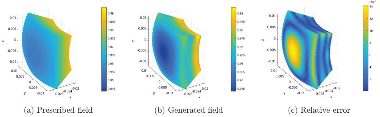
Figure 5: Results of the field synthesis on the near control
