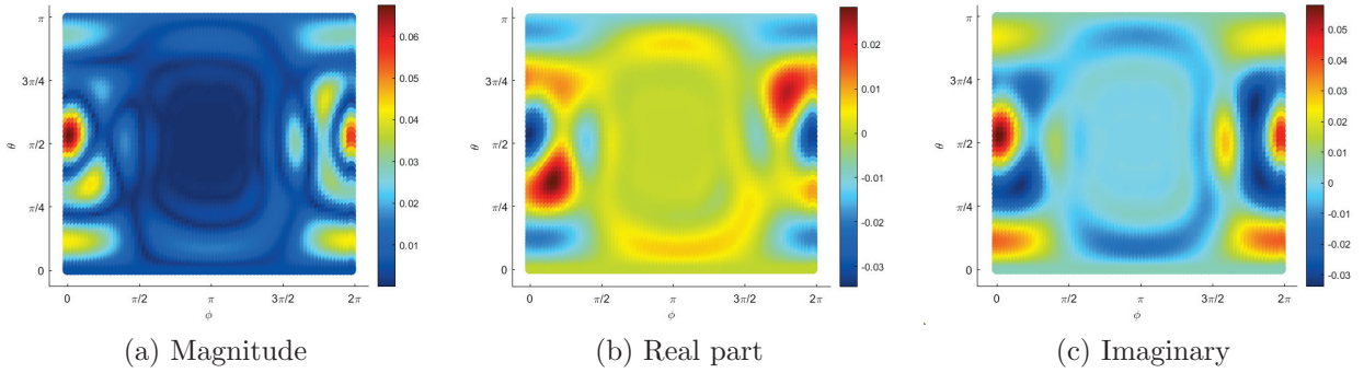
Figure 7: The computed normal velocity on the actual source
