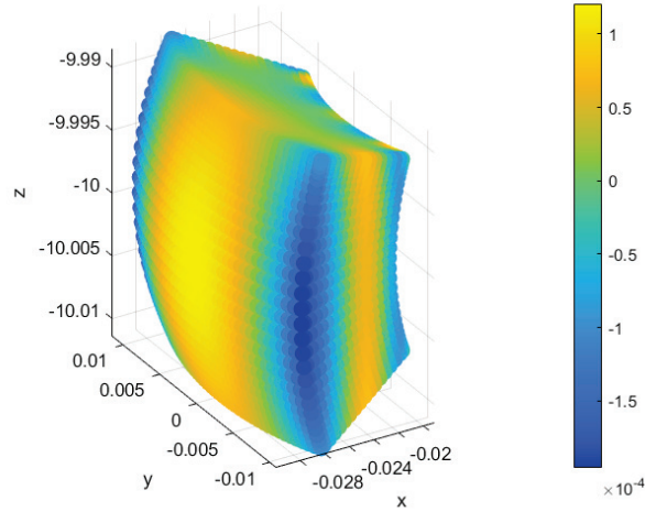
Figure 11: Real part of the generated near field
