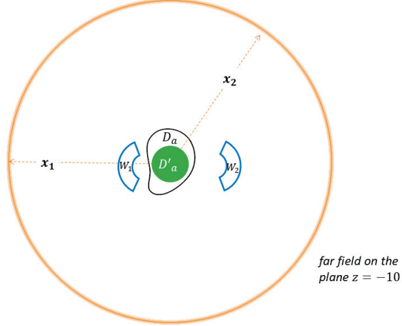
Figure 17: A cross section of the simulation geometry
