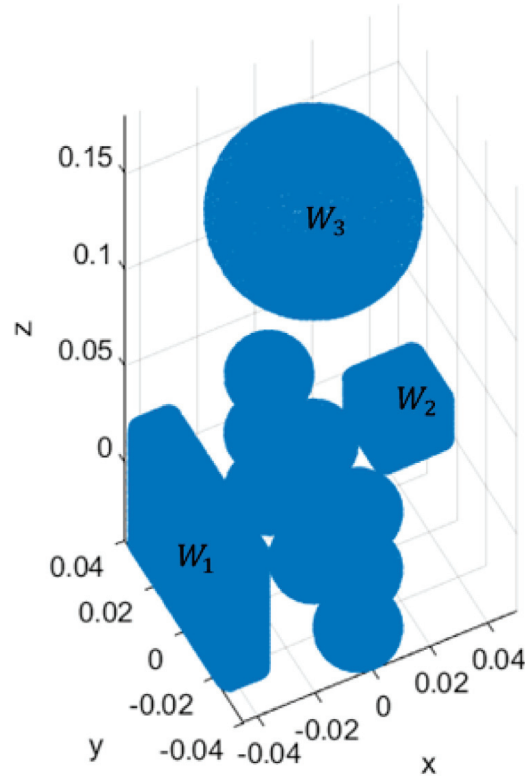
Fig. 7. Illustration of the simulation geometry.
