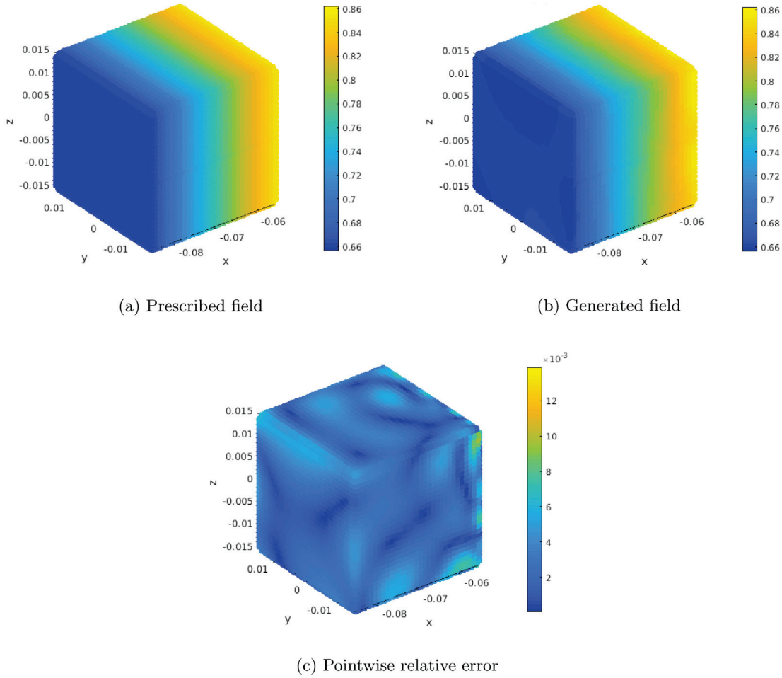
Fig. 13. Results of the pattern synthesis on W_1 .
