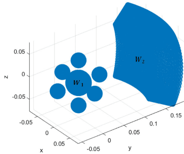
Fig. 21. Illustration of the simulation geometry.
