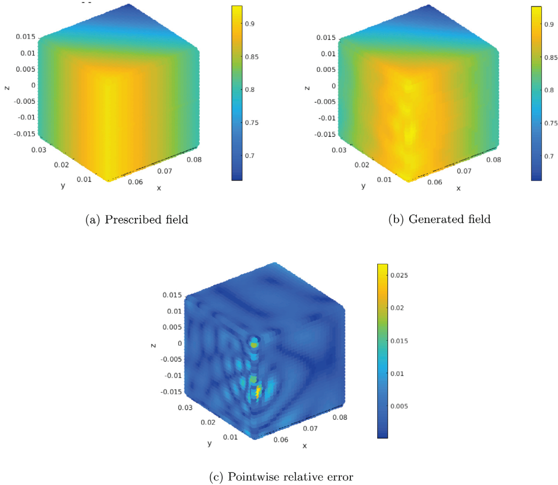
Fig. 14. Results of the pattern synthesis on W_2 .
