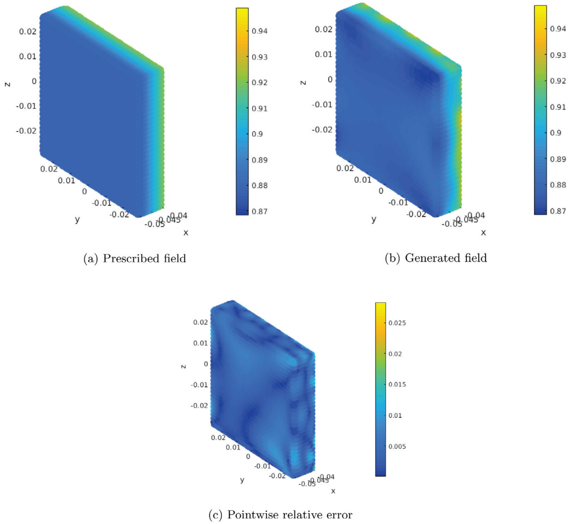
Fig. 8. Results of the pattern synthesis on W_1 .
