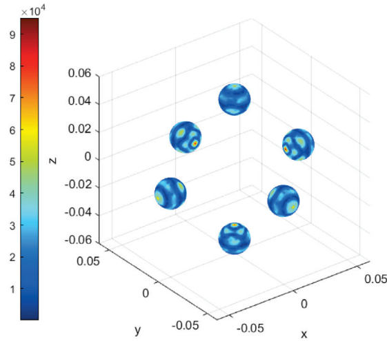
Fig. 20. Pointwise magnitude of the density w .
