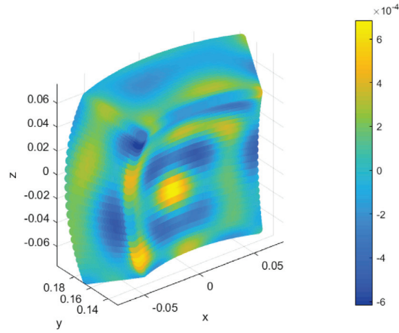
Fig. 26. Real part of the generated field on W_2 .
