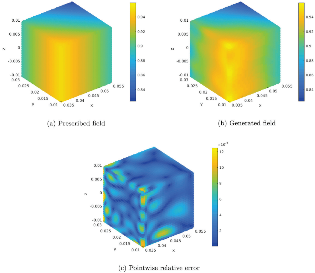
Fig. 9. Results of the pattern synthesis on W_2 .
