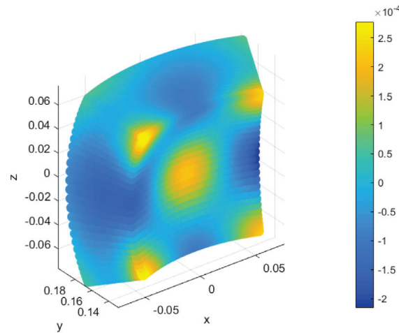
Fig. 23. Real part of the generated field on W_2 .
