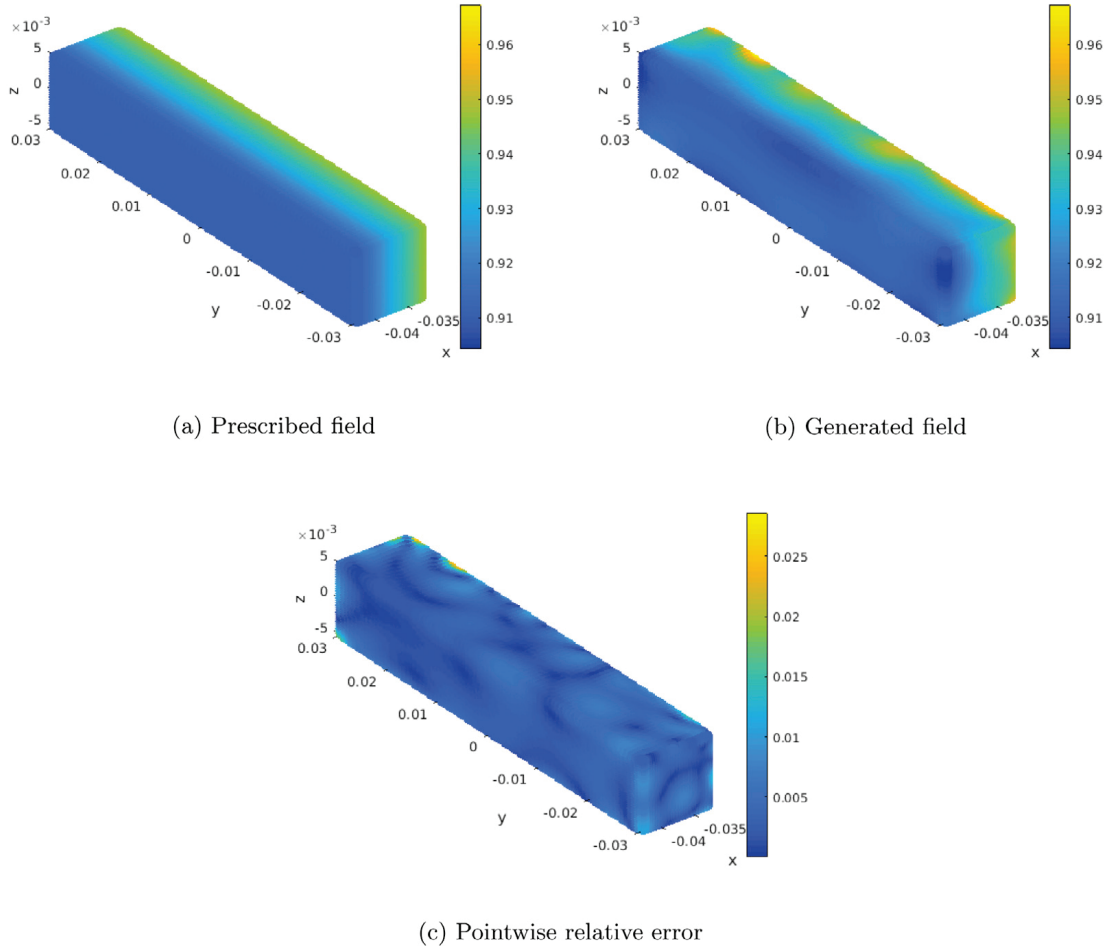
Fig. 3. Results of the pattern synthesis on W_1 .
