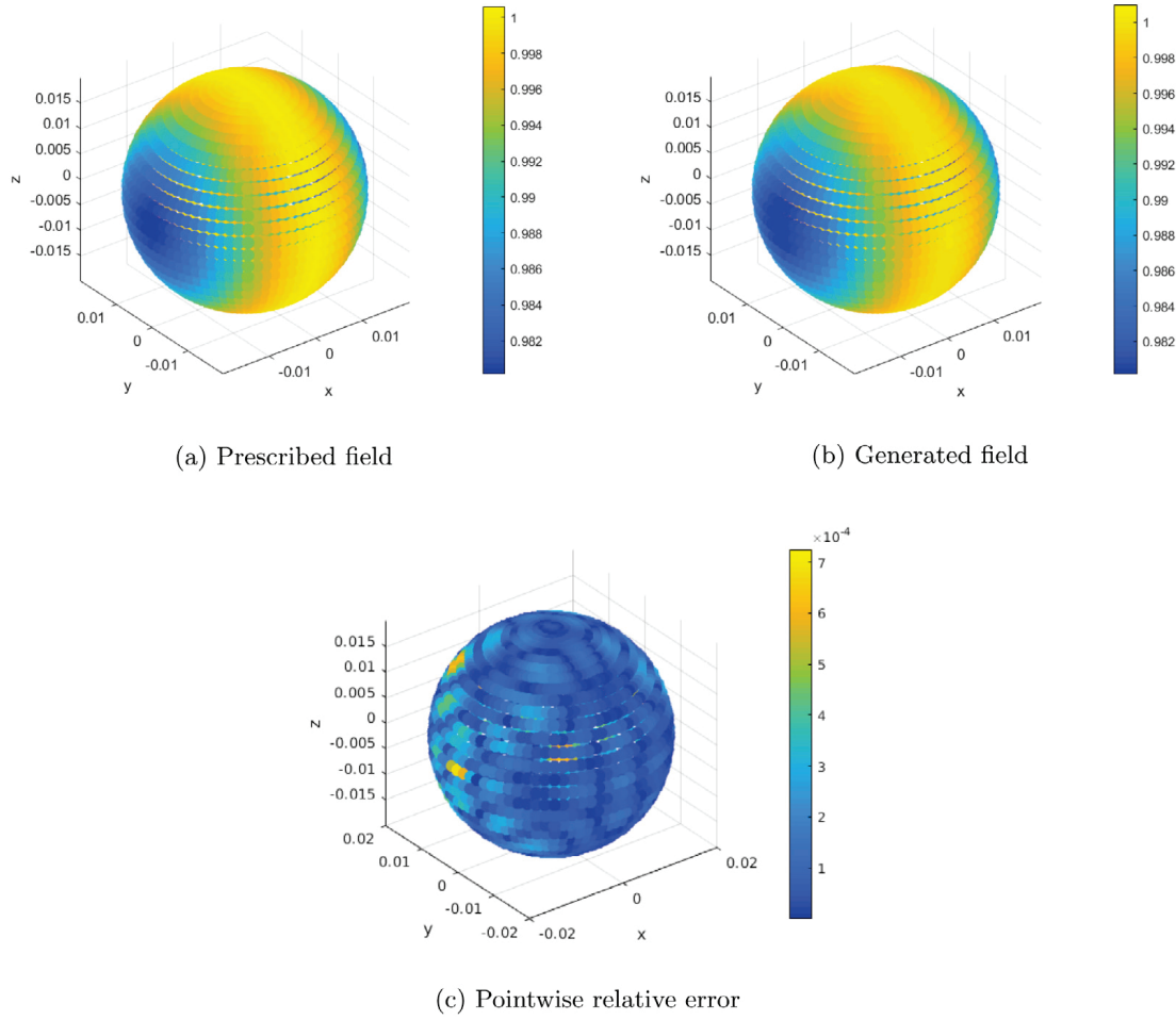
Fig. 22. Results of the pattern synthesis on W_1 .
