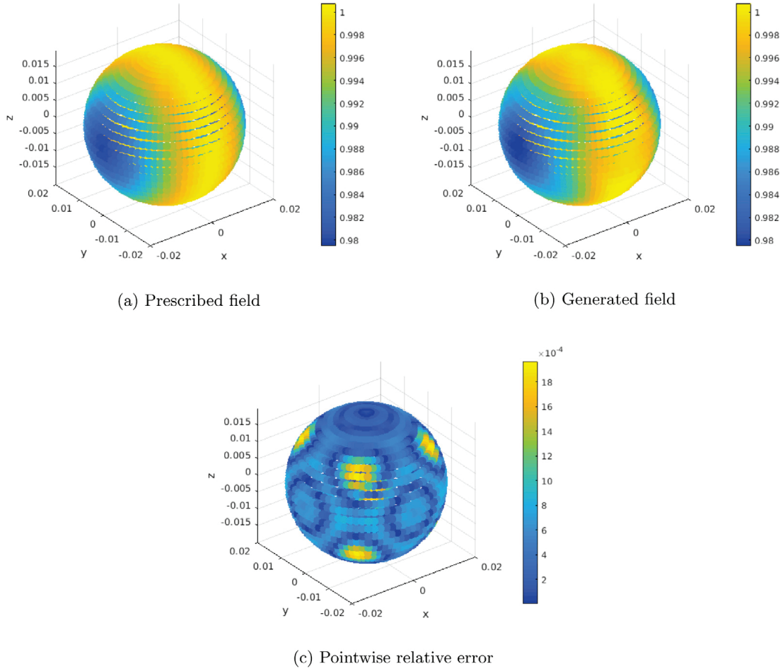
Fig. 18. Results of the pattern synthesis on W_1 .
