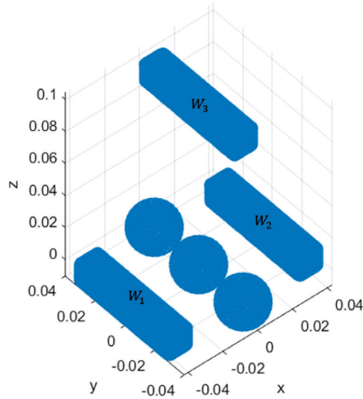
Fig. 2. Illustration of the simulation geometry.
