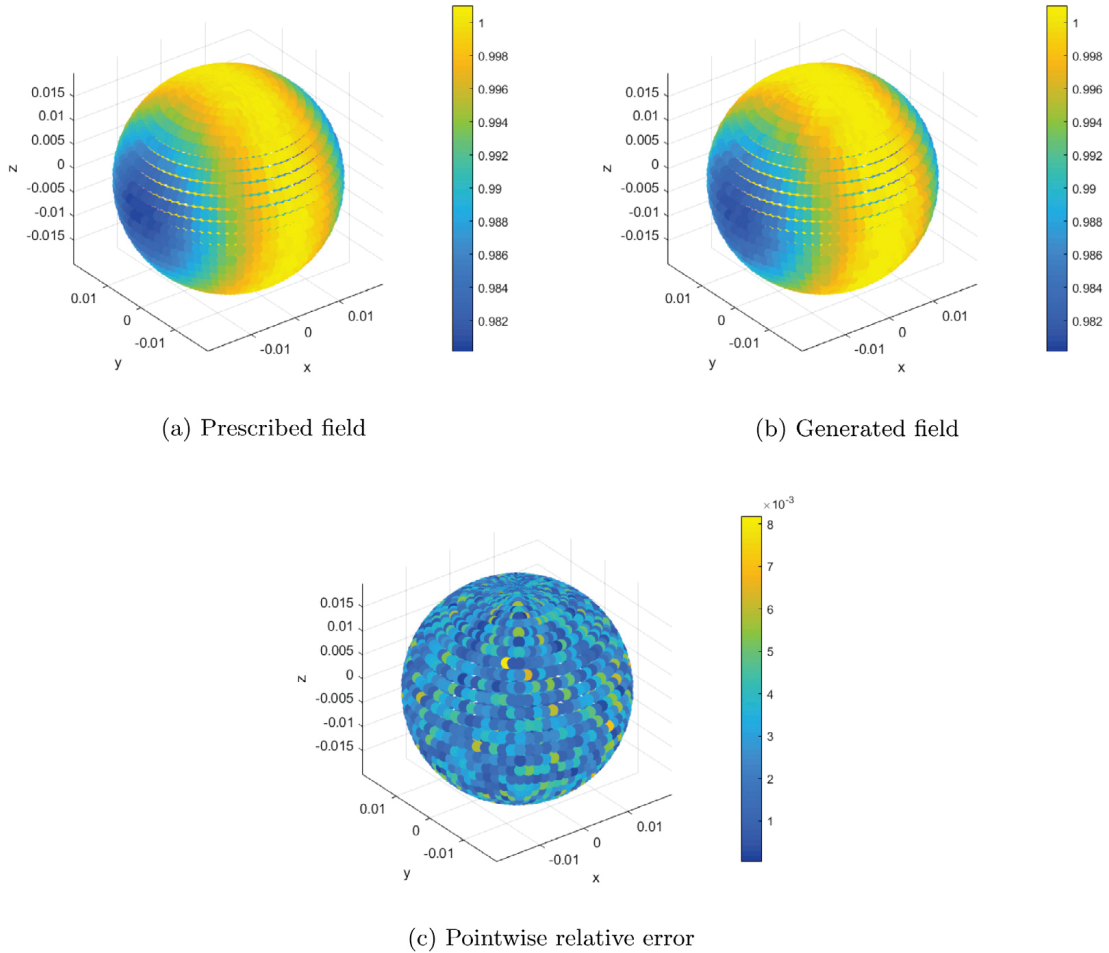
Fig. 25. Results of the pattern synthesis on W_1 .
