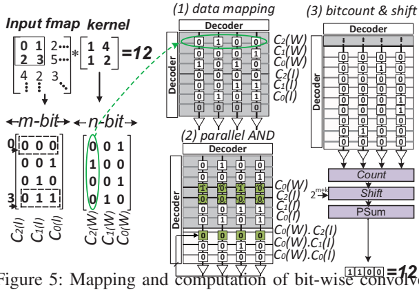
Figure 5: Mapping and computation of bit-wise convolver.
