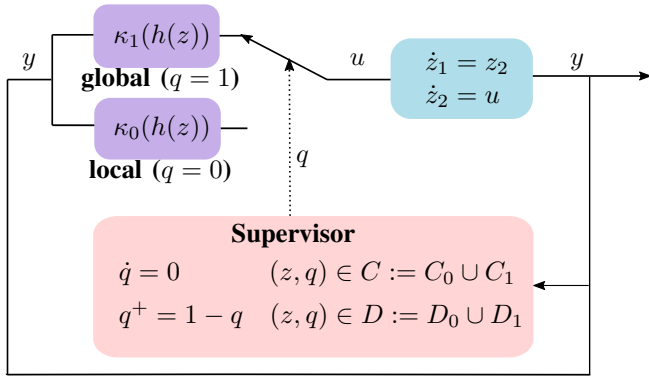
Fig. 2. Feedback diagram of the hybrid closed-loop system \mathcal{H} , in (7), uniting global and local optimization algorithms.
