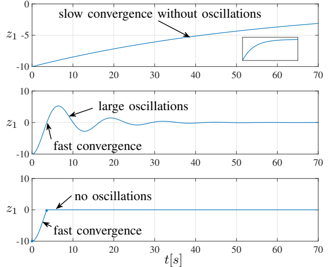
Fig. 1. Comparison of the performance of the heavy ball method, with large and small values of \lambda , and with proposed logic-based algorithm for L(z_1) = \frac{1}{4}z_1^2 . Top: when \lambda is large, heavy ball converges very slowly (zoomed out plot included). Middle: when \lambda is small, heavy ball converges quickly, but with wild oscillations. Bottom: our proposed logic-based strategy yields fast convergence, with no oscillations.
