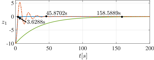
Fig. 4. A comparison of the evolution of z_1 over time for \mathcal{H}_0 , \mathcal{H}_1 , and \mathcal{H} – which uses measurements of \nabla L(z_1) – for L(z_1) = \frac{1}{4}z_1^2 , with a single minimum at \mathcal{A}_1 = \{0\} . The global heavy ball algorithm \mathcal{H}_1 uses \lambda_1 = \frac{1}{5} and \gamma_1 = \frac{1}{2} (shown in red) and settles to within a 1% margin of \mathcal{A}_1 in about 45.9 seconds. The local heavy ball algorithm \mathcal{H}_0 uses \lambda_0 = 11.5 and \gamma_0 = \frac{2}{3} (shown in green) and settles to within 1% of \mathcal{A}_1 in about 158.6 seconds. The hybrid closed-loop system \mathcal{H} (shown in blue) settles to within 1% of \mathcal{A}_1 in about 3.6 seconds.
