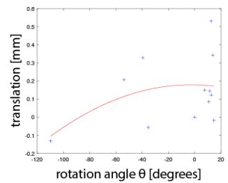
Fig. 11. Fitting the residual \hat{x} .
