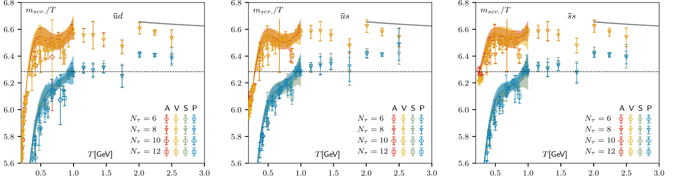
FIG. 9. Screening masses divided by the temperature, for temperatures T \gtrsim 200 MeV and for N_\tau = 6, 8, 10, and 12 for all four channels in different flavor sectors. The gray curve in the top right part of each figure is the resummed perturbation theory prediction [67,68]. The horizontal dashed line in each plot is the infinite-temperature limit m_{\text{scr}}^{\text{free}}/T = 2\pi . Both the infinite-temperature limit as well as the perturbative result are the same for all screening masses irrespective of their spin. Beyond T \gtrsim 1 GeV, only N_\tau = 8 data exist as a result of which a continuum extrapolation is not possible. The lattice results are obtained with corner wall source for V and AV channels for T \lesssim 300 MeV and with point source elsewhere.
