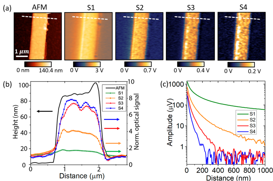
Figure 1. Assessment of spatial resolution and signal-to-noise ratio obtained via THz s-SNOM. (a) Left to right: AFM topographic image and near-field images demodulated at different harmonics of the tip's tapping frequency. (b) Height and near-field optical signal profiles along the white dashed lines in (a). S1 through S4 are normalized to the average substrate signal in their corresponding images to yield a relative contrast. (c) Approach curves for different orders of demodulation on gold bar.
