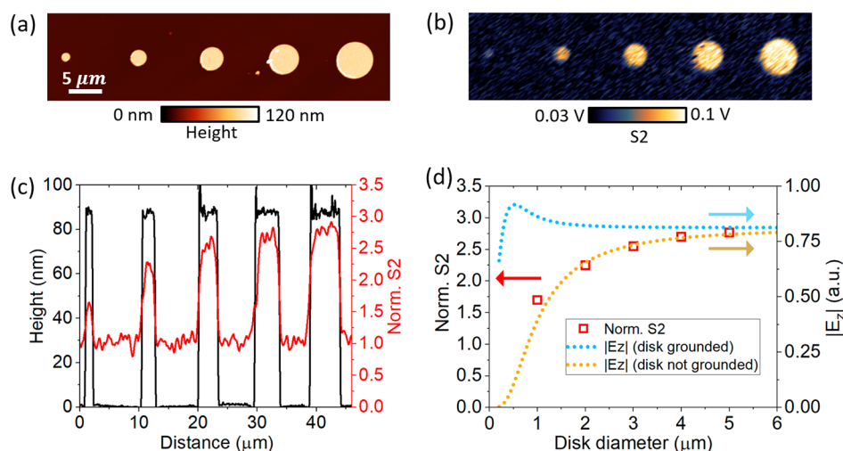
Figure 2. (a) AFM image of a series of micron-sized gold disks. (b) The corresponding second harmonic near-field amplitude image at 171.84 GHz (1.74 nm), which shows an increasing near-field response with increasing disk diameter. (c) Height and normalized near-field S2 optical signal profiles across the disks in (a) and (b). The height of the disk is constant ( \sim 80 nm), while S2 increases with increasing disk diameter. (d) Red squares: average and normalized near-field signal (S2) of the disks with different diameters. Brown and blue curves represent the calculated electric field at the point charge for ungrounded and grounded disks, respectively.
