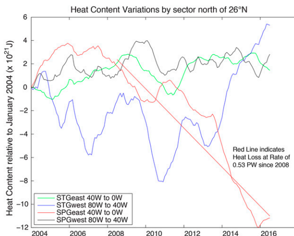
FIG. 5. Temporal variability in ocean heat content north of 26^{\circ} N for four regions: Subtropical Gyre East ( 26^{\circ} – 40^{\circ} N, 40^{\circ} W– 0^{\circ} ), Subtropical Gyre West ( 26^{\circ} – 40^{\circ} N, 80^{\circ} – 40^{\circ} W), Subpolar Gyre East ( 40^{\circ} – 70^{\circ} N, 40^{\circ} W– 0^{\circ} ), and Subpolar Gyre West ( 40^{\circ} – 70^{\circ} N, 80^{\circ} – 40^{\circ} W). Differences from 2004 values are shown for each region. EN4 gridded temperature and salinity fields updated from Good et al. (2013) are used. The red line indicates ocean heat loss at a rate of 0.053 PW based on a least squares estimate of the slope in heat content change since 2008. Estimated uncertainty in this change for Subpolar Gyre East is 0.018 PW, assuming independent values every 12 months.
