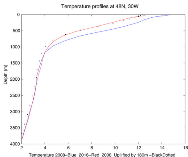
FIG. 9. Temperature profiles at 48°N, 30°W in 2008 (blue) and 2016 (red) based on EN4 data updated from Good et al. (2013). The black dots indicate 2008 profile uplifted by 180 m to show that the thermocline in the eastern subpolar gyre has risen since 2008.
