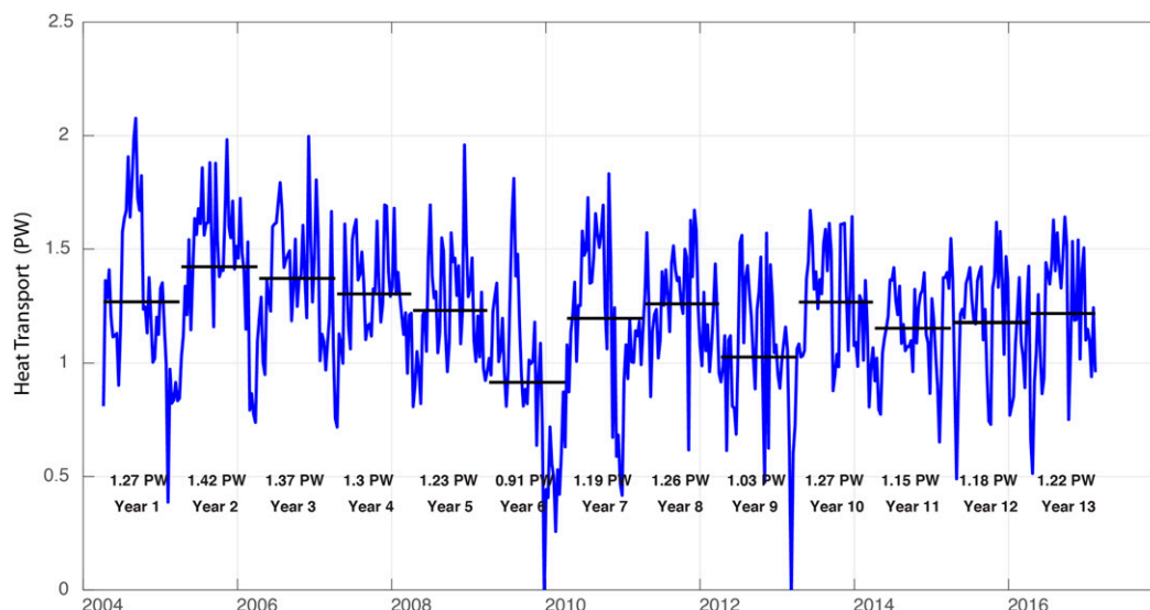
FIG. 2. Ocean heat transport at 26°N from RAPID measurements. Ten-day filtered values following the method in Johns et al. (2011) are shown. Horizontal black lines indicate annual average values (April–March) for each year. Northward ocean heat transport averages 1.32 PW for 2004–09 but only 1.15 PW after 2009. There is a decrease in ocean heat transport of 0.17 PW resulting from the reduction in the AMOC during late 2008 and early 2009.
