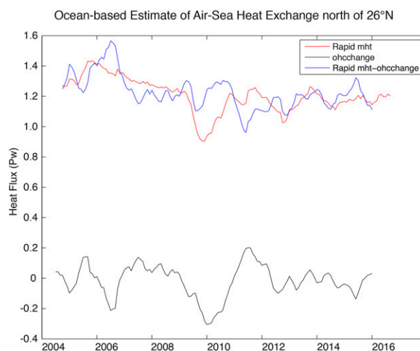
FIG. 11. Ocean heat transport at 26°N (red), ocean heat content change (black), and their sum (blue), which is equal to the ocean heat loss to the atmosphere north of 26°N. The sum represents an ocean-based estimate of ocean heat loss for the Atlantic between 26° and 70°N.
