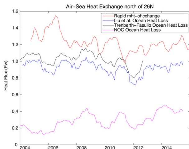
FIG. 12. Comparison of ocean-based estimates of ocean heat loss north of 26^{\circ}\text{N} with recent climatologies of air–sea exchange. The ocean-based estimate from Fig. 11 is equal to the northward heat transport at 26^{\circ}\text{N} from RAPID measurements minus ocean heat content change north of 26^{\circ}\text{N} from EN4 values for heat content; J. Fasullo provided the ocean heat loss estimates from TF17, C. Liu provided the values of ocean heat loss from L17, and E. Kent provided the NOC ocean heat loss based on ship of opportunity measurements [updated from Berry and Kent (2011)].
