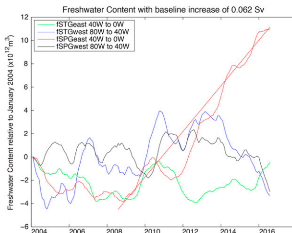
FIG. 7. Temporal variability in ocean freshwater content north of 26^\circ\text{N} for four regions: Subtropical Gyre East ( 26^\circ – 40^\circ\text{N} , 40^\circ\text{W} – 0^\circ ), Subtropical Gyre West ( 26^\circ – 40^\circ\text{N} , 80^\circ – 40^\circ\text{W} ), Subpolar Gyre East ( 40^\circ – 70^\circ\text{N} , 40^\circ\text{W} – 0^\circ ), and Subpolar Gyre West ( 40^\circ – 70^\circ\text{N} , 80^\circ – 40^\circ\text{W} ). Differences from 2004 values are shown for each region. EN4 gridded temperature and salinity fields updated from Good et al. (2013) are used. The red line indicates an increase in ocean freshwater at a rate of 0.062 Sv based on a least squares estimate of the slope in freshwater content change since 2008 in the eastern subpolar gyre. Estimated uncertainty in this change for Subpolar Gyre East is 0.013 Sv, assuming independent values every 12 months.
