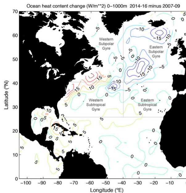
FIG. 4. Ocean heat content change ( \text{W m}^{-2} ) for 2014–16 minus 2007–09. EN4 gridded temperature and salinity fields updated from Good et al. (2013) are used.
