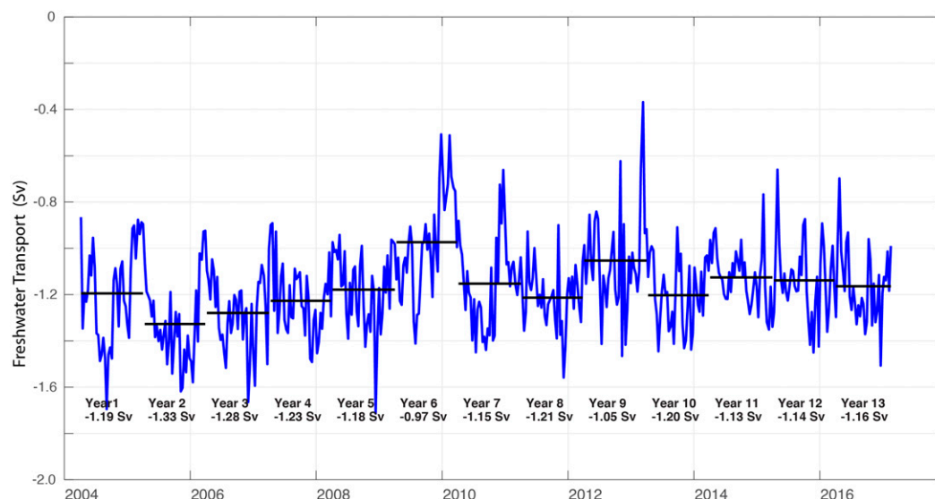
FIG. 3. Freshwater transport across 26°N from RAPID measurements. Ten-day filtered values following the method in McDonagh et al. (2015) are shown. Horizontal black lines indicate annual average values (April–March) for each year. Southward freshwater transport during 2004–09 averages 1.24 Sv. As a result of the reduction in the AMOC in late 2008 and early 2009, southward freshwater transport after 2009 averages only 1.13 Sv. There is an increase in northward freshwater transport across 26°N of 0.12 Sv from before 2009 to after 2010.
