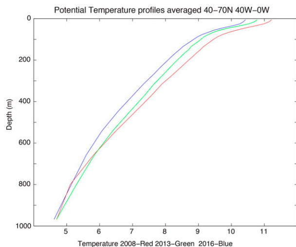
FIG. 10. Potential temperature profiles. Annual average temperatures from EN4 updated from Good et al. (2013) are averaged over the eastern subpolar region 40°–70°N, 40°W–0° for 2008, 2013, and 2016 to show persistent cooling from 2008 to 2016. Here, 2013 is chosen because it is before the severe winters of 2014 and 2015 and it indicates cooling since 2008 down to 650 m. The severe winter mixing in 2014 and 2015 led to cooling down to 800 m.
