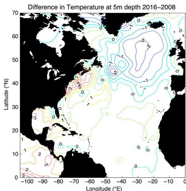
FIG. 8. Difference in temperature at 5-m depth (2016 minus 2008) based on EN4 annual average temperatures updated from Good et al. (2013). Surface temperatures are 2°C colder over 8 years in the midocean region south of Iceland.
