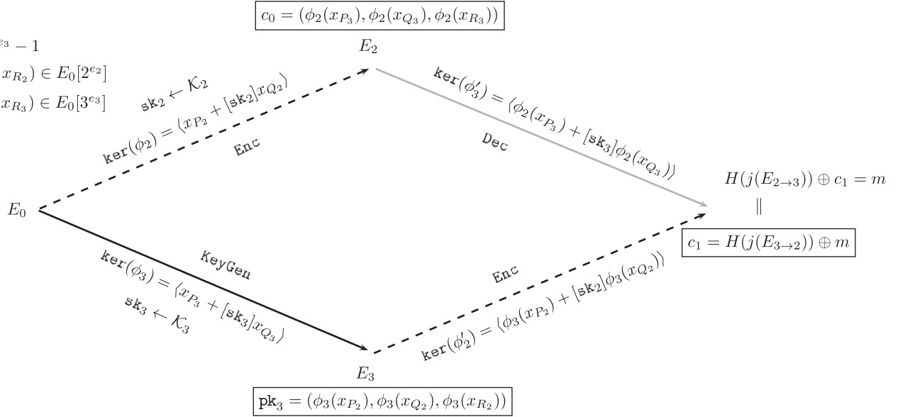
Fig. 1. Supersingular isogeny PKE protocol.
