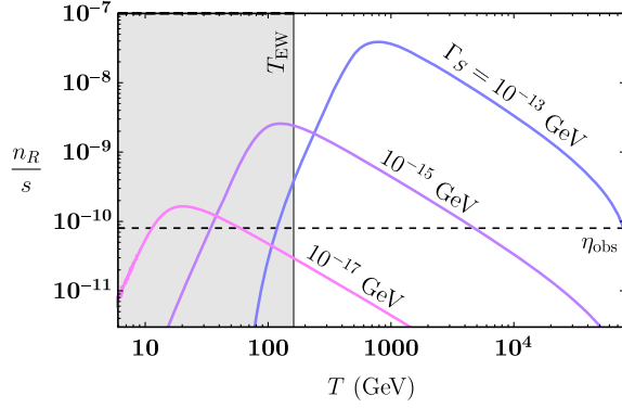
FIG. 3. Right-handed electron asymmetry generated through asymmetric flavon decays for different values of the flavon decay rate \Gamma_S . The observed baryon asymmetry \eta_{\text{obs}} \simeq 8 \times 10^{-11} is shown for reference.
