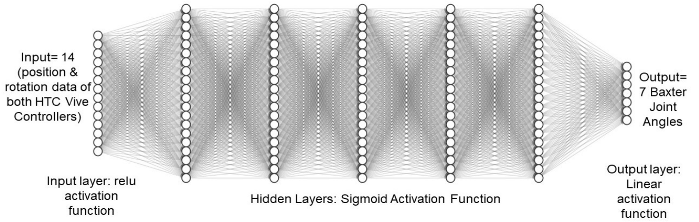
Fig. 2. Training of the deep neural network to learn the correspondence between the Baxter robot joint angles and the human poses where input 14 represents the position and rotation data of HTC Vive controller placed in two respective hand of the human demonstrator and output 7 represents the seven joint angles of one of the Baxter robot’s arm.
