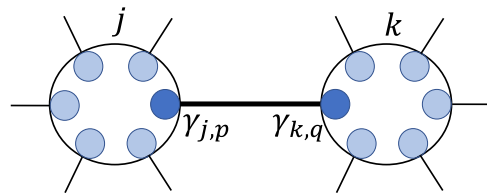
FIG. 1. Local Majorana modes for nearest-neighbor vertices j, k . We define \tilde{A}_{j,k} = \epsilon_{j,k} \gamma_{j,p} \gamma_{k,q} , where \epsilon_{j,k} = \pm 1 is the edge orientation. The operator \tilde{B}_j is proportional to the product of all local Majorana modes \gamma_{j,p} located at the vertex j .
