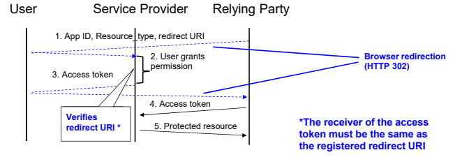
Fig. 2: Overview of OAuth 2.0.
