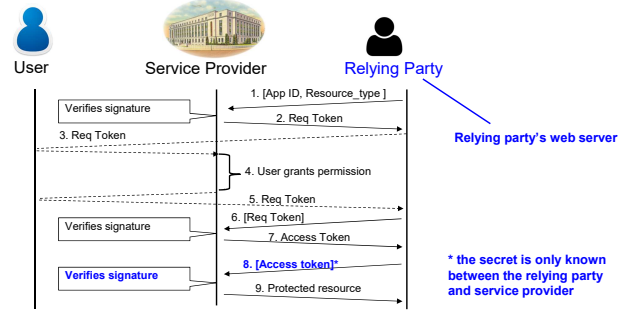
Fig. 1: Overview of OAuth 1.0.
