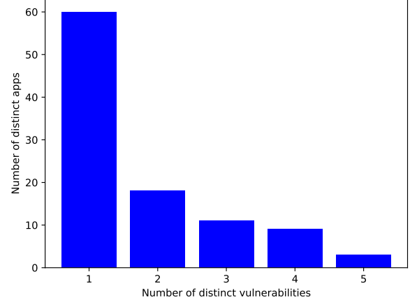
Fig. 9: Number of applications with 1, 2, ...5 vulnerabilities.
