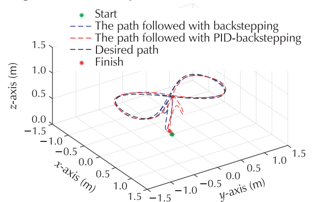
Fig. 8 The path tracked by the UAV with backstepping controller and backstepping controller with PID tracker using 8-figure trajectory.
