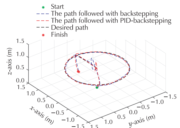
Fig. 9 The path tracked by the UAV with backstepping controller and backstepping controller with PID tracker using circular trajectory.
