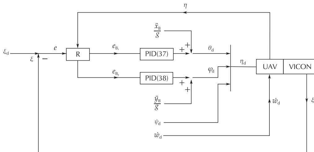
Fig. 3 Tracker design of backstepping controller using PID control method.
