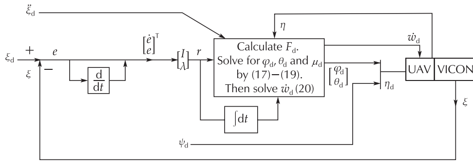
Fig. 2 Tracker design of backstepping controller using sliding variable.
