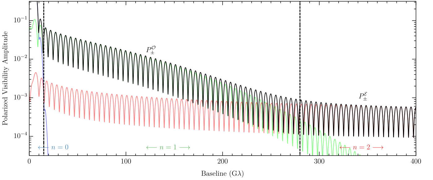
FIG. 3. Schematic showing polarized visibility amplitude as a function of baseline length for a photon ring with d = 40 \mu\text{as} . Visibility amplitudes are shown for the complete image (black) as well as for individual subrings ( n = 0 : blue, 1: green, 2: red). Progressively longer baselines are dominated by visibilities for a subring with correspondingly larger index n . The visibility amplitudes in each range are determined by a pair of complex coefficients, P_{\pm}^O or P_{\pm}^E depending upon whether n is odd or even. The periodicity of the visibility amplitudes gives the subring diameter in the baseline direction, while the coefficients P_{\pm}^O and P_{\pm}^E carry information about the black hole spin and azimuthal brightness asymmetry.
