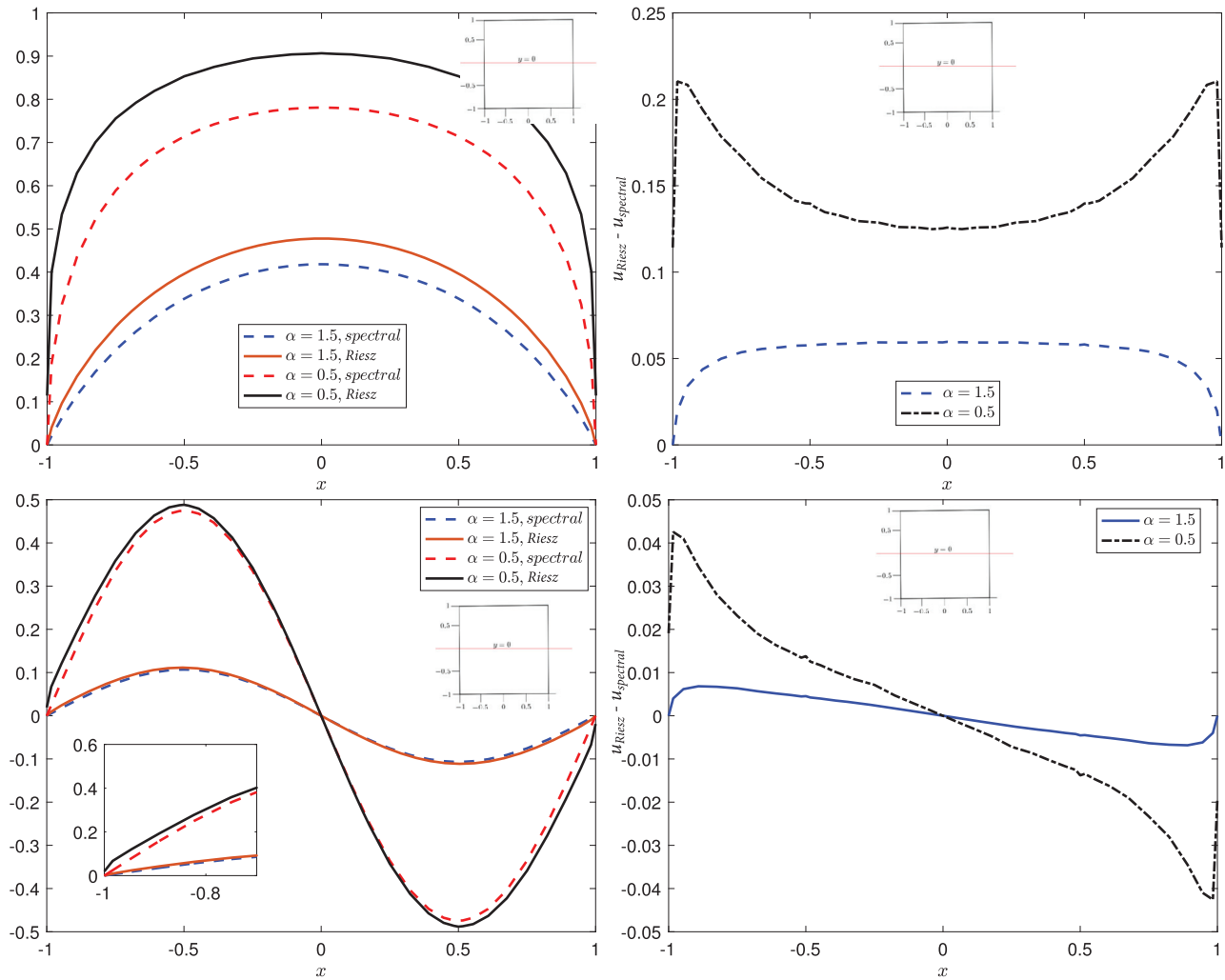
Fig. 17. Slices along the line y=0 in the square domain with both \alpha=0.5 and \alpha=1.5 . (top left) Plots of the solutions for the Riesz and spectral formulations with f=1 and (top right) plot of the differences u_{\text{Riesz}} - u_{\text{spectral}} along the line y=0 with f=1 . (bottom left) Plots of the solutions for the Riesz and spectral formulations with f=\sin(\pi x)\sin(\pi y) and (bottom right) plot of the differences u_{\text{Riesz}} - u_{\text{spectral}} along the line y=0 with f=\sin(\pi x)\sin(\pi y) . Some small wiggles that appear in the difference plots are due to the computation of the differences on two different meshes, even though the solutions are sufficiently converged and stable.
