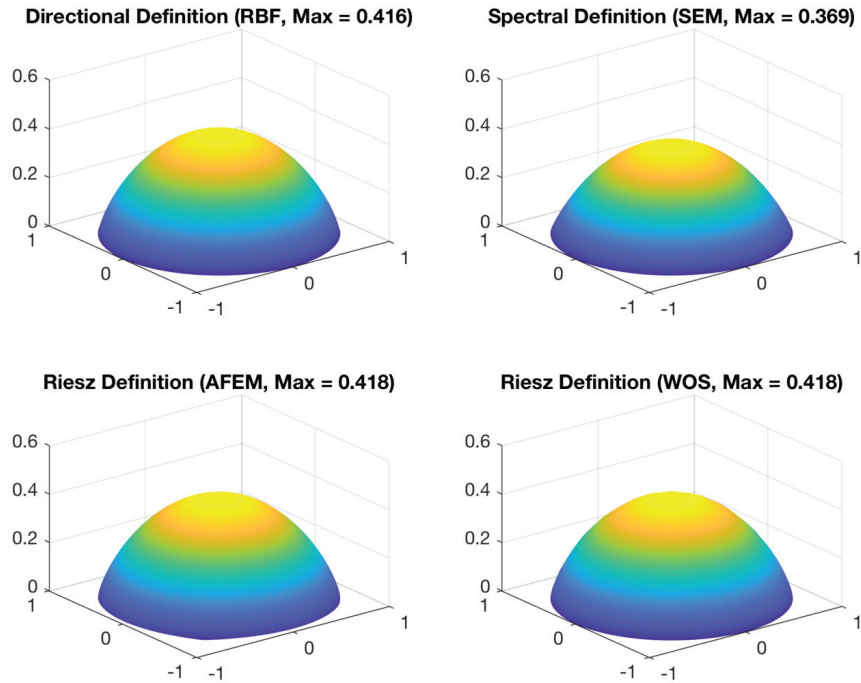
Fig. 35. Unit disk, f = 1 , and g(x) = 0 : Comparison, for \alpha = 1.5 , of u_{Riesz} and u_{spectral} , using three methods to compute the Riesz solution and one method to compute the spectral solution. Top left : The Riesz solution obtained using the RBF collocation method based on the directional representation. Top right : The spectral solution obtained using the SEM. Bottom left : The Riesz solution obtained using the AFEM. Bottom right : The Riesz solution obtained using the WOS method. The only solution with a significant difference is the spectral solution ( top right ); all other solutions are equivalent up to numerical error.
