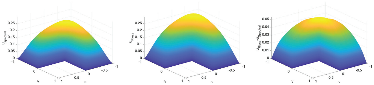
(d) Solutions u associated with f = 1 and \alpha = 1.5 in the L-shaped domain using the spectral definition (using SEM) ( left ) and the Riesz definition (using AFEM) ( center ), and the difference between u_{\text{Riesz}} and u_{\text{spectral}} for this case ( right ).
