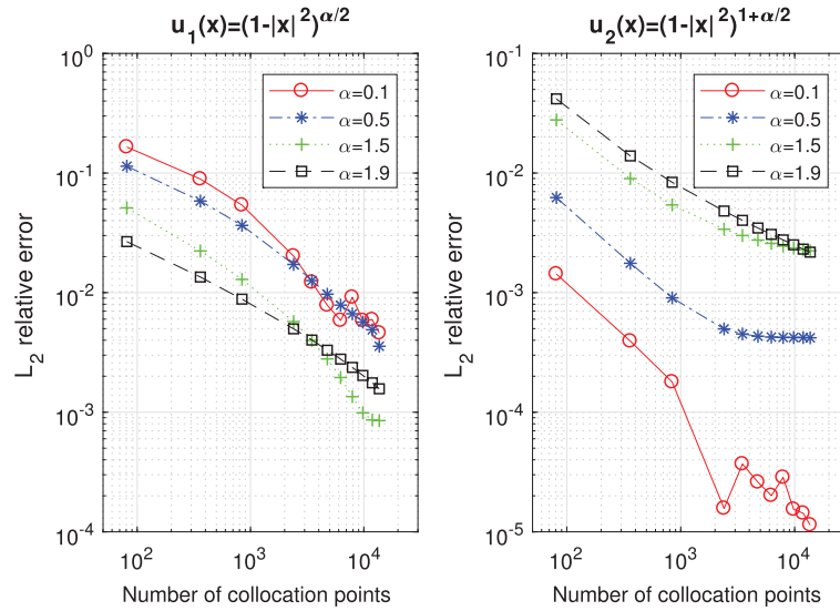
Fig. 8. Convergence of the RBF method for the 2D fractional Poisson problem with zero exterior values on a unit disk. Left: fabricated solution u_1 with \alpha = 0.1, 0.5, 1.5 , and 1.9 . Right: fabricated solution u_2 with \alpha = 0.1, 0.5, 1.5 , and 1.9 .
