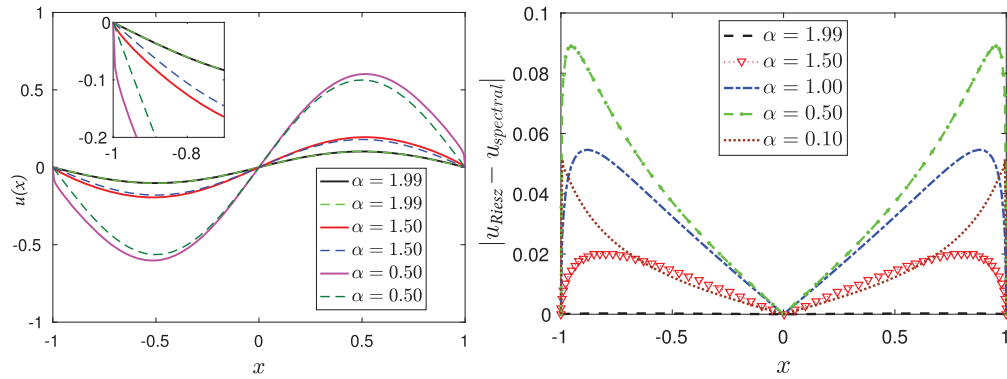
Fig. 4. One-dimensional study: (left) The numerical solutions of both the spectral and Riesz fractional Poisson equations with f = \sin(\pi x) . The solid curves are solutions of the spectral Poisson equation computed with the spectral element method where \mathcal{N} = 64 . The dashed curves represent the solutions of the Riesz fractional Poisson equation which are computed using a finite element approximation. (right) The absolute differences between the spectral solutions u_{\text{spectral}} and the Riesz solutions u_{\text{Riesz}} of their respective fractional Poisson equations for the smooth right-hand-side f = \sin(\pi x) on the interval (-1, 1) .
