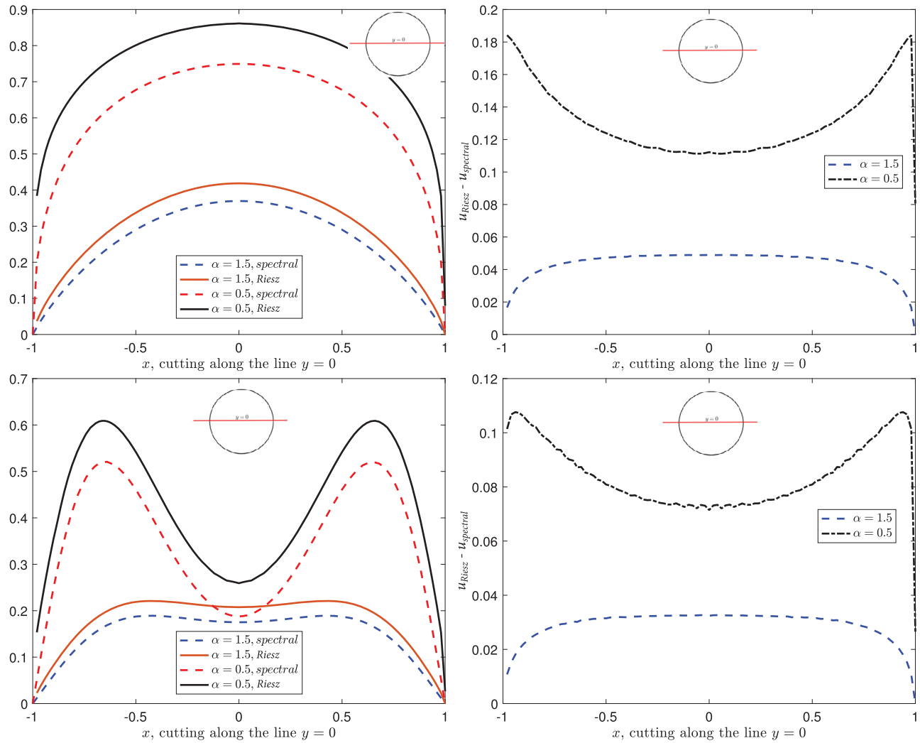
Fig. 20. Slices along the line y=0 in the unit disk domain with both \alpha=0.5 and \alpha=1.5 . (top left) Plots of the solutions for the Riesz and spectral formulations with f=1 and (top right) plot of the differences u_{\text{Riesz}} - u_{\text{spectral}} along the line y=0 and f=1 . (bottom left) Plots of the solutions for the Riesz and spectral formulations with f=\sin(\pi r^2) and (bottom right) plot of the differences u_{\text{Riesz}} - u_{\text{spectral}} along the line y=0 and f=\sin(\pi r^2) . Some small wiggles that appear in the difference plots are due to the computation of the differences on two different meshes, even though the solutions are sufficiently converged and stable.
