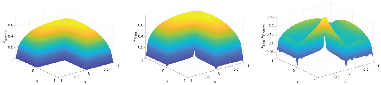
(c) Solutions u associated with f = 1 and \alpha = 0.5 in the L-shaped domain using the spectral definition (using SEM) ( left ) and the Riesz definition (using AFEM) ( center ), and the difference between u_{\text{Riesz}} and u_{\text{spectral}} for this case ( right ).
