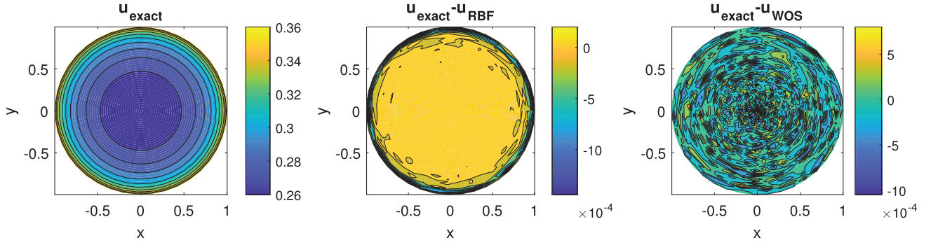
(a) Exact vs RBF vs WOS solutions
