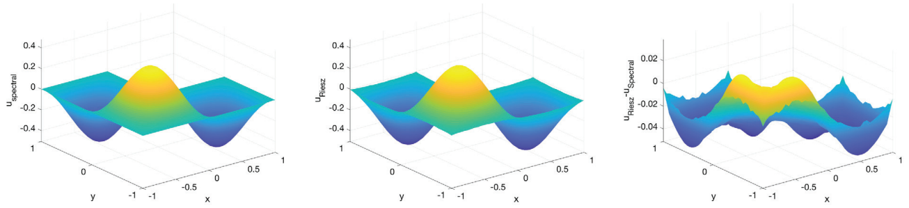
(a) Solutions u associated with f = \sin(\pi x)\sin(\pi y) and \alpha = 0.5 in the L-shaped domain using the spectral definition (using SEM) (left) and the Riesz definition (using AFEM) (center), and the difference between u_{\text{Riesz}} and u_{\text{spectral}} for this case (right).
