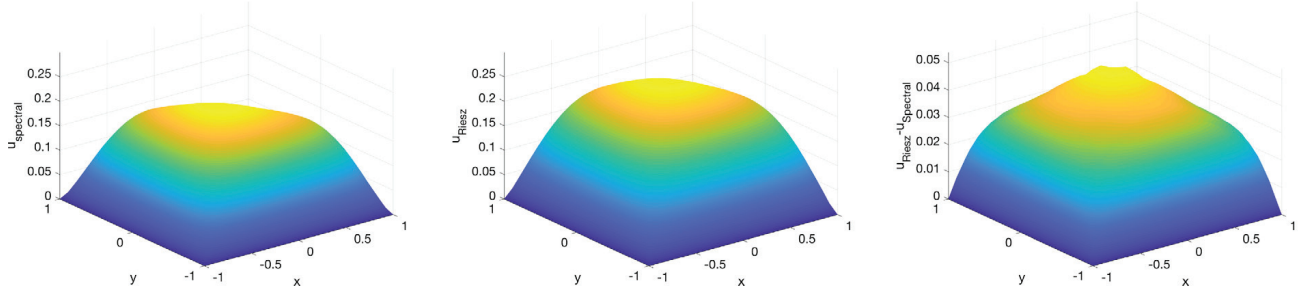
(b) Solutions u associated with f = 1 and \alpha = 1.5 in the L-shaped domain using the spectral definition (using SEM) ( left ) and the Riesz definition (using AFEM) ( center ), and the difference between u_{\text{Riesz}} and u_{\text{spectral}} for this case ( right ).
