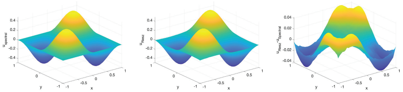
(a) Solutions u associated with f = \sin(\pi x) \sin(\pi y) and \alpha = 0.5 in the square domain using the spectral definition (using SEM) (left) and the Riesz definition (using AFEM) (center), and the difference between u_{\text{Riesz}} and u_{\text{spectral}} for this case (right).
