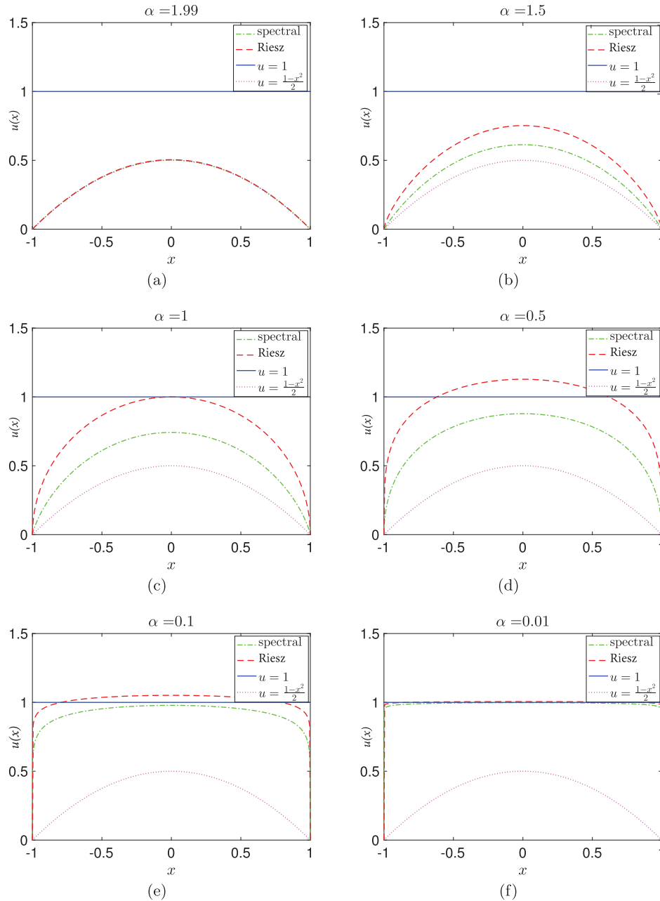
Fig. 1. One-dimensional study: The profiles of the numerical solutions of (1) for different fractional orders \alpha : (a)–(f) for \alpha = 1.99, 1.5, 1.0, 0.5, 0.1, 0.01 . The pink dotted curve corresponds to the solution in the case \alpha = 2 , and the blue line represents the (discontinuous) solution for \alpha = 0 , and are included for reference. Note that the Riesz solution has greater amplitude than the spectral solution, and this amplitude increases above u = 1 as \alpha goes to zero before decreasing to one in the plot for \alpha = 0.01 . (For interpretation of the colors in the figure(s), the reader is referred to the web version of this article.)
