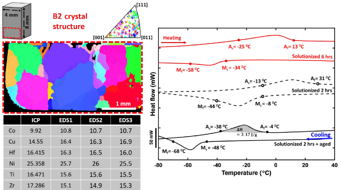
Fig. 1. Sample geometry and EBSD scan of the region indicated with a red rectangle confirming cubic B2 structure, grain size and diversity of grain distribution. The stereographic triangle shown is for the loading direction. The table presents composition results from ICP as well as three different EDS scans along the specimen. DSC scans are presented on the right. The solid black line corresponds to the solutionized for 2 h + aged case. The dashed black line represents the solutionized (2 h) only case and the solid red line the longer 6-h solutionizing treatment. The corresponding characteristic temperatures are marked on the figure. Solutionized only results are scaled up 5 times to aid the eye. DSC heating/cooling rate used was 20 °C/min.
