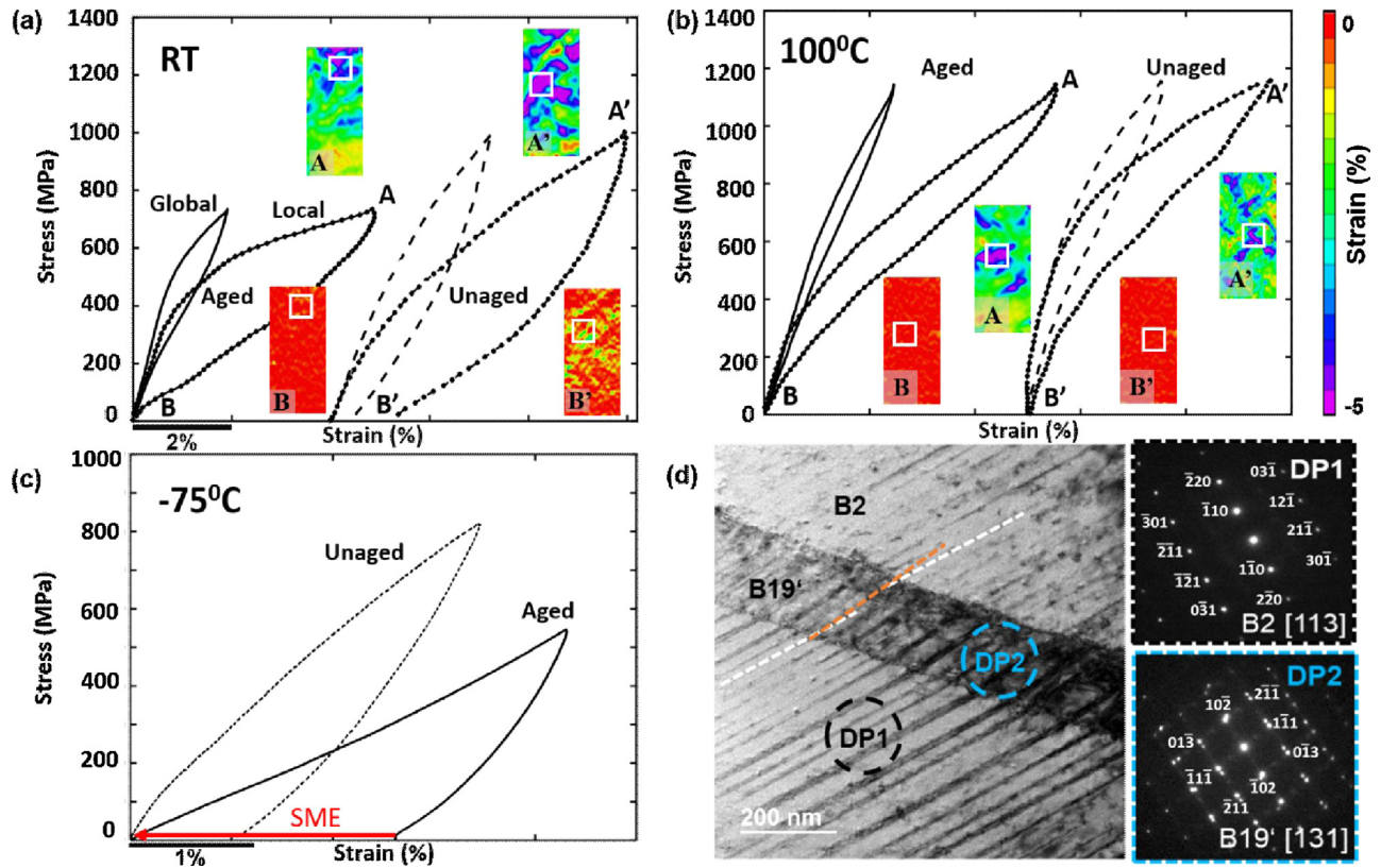
Fig. 2. Compressive stress strain behavior of (\text{TiZrHf})_{50}\text{Ni}_{25}\text{Co}_{10}\text{Cu}_{15} in unaged and aged conditions at (a) room temperature and (b) 100 °C, strain scale bar is 2%. The DIC insets cover the entire specimen surface ( 4 \times 8 \text{ mm}^2 ) and the white boxes indicate the localization area from which local strains were extracted. The compressive stress strain response at -75 °C is shown in (c), strain scale bar is 1%. The TEM bright field image and corresponding diffraction patterns in (d) obtained after compressive testing at room temperature (25 °C) show retained, internally twinned martensite (B19') within the austenitic matrix (B2) and slip emanating from the martensite twins into the austenite.
