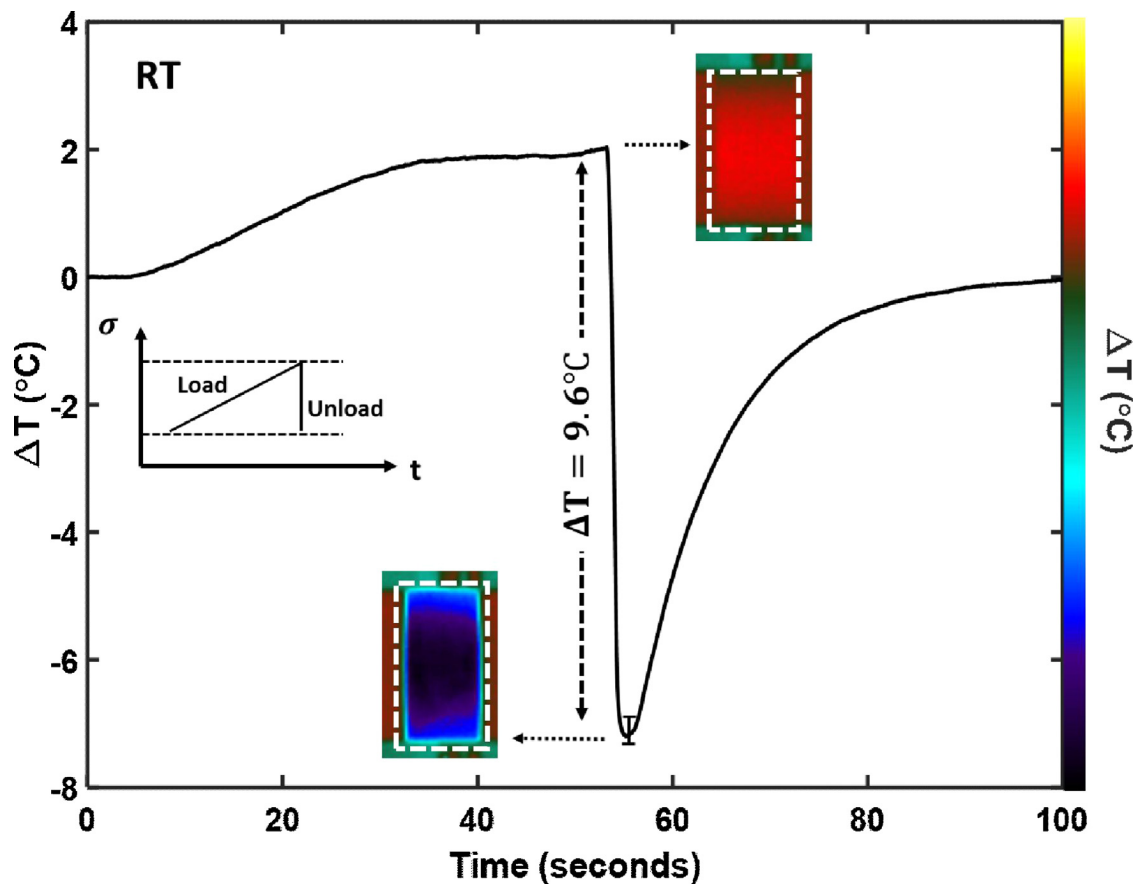
Fig. 4. Infrared IR temperature signature during an asymmetric double ramp loading (the inset shows slow loading and rapid unloading) cycle for an aged sample at room temperature for \text{Ti}_{16.67}\text{Zr}_{16.67}\text{Hf}_{16.67}\text{Ni}_{25}\text{Co}_{10}\text{Cu}_{15} . Color scale bar on right hand side corresponds to the same \Delta T scale on left side of the figure. Multiple tests were conducted and the error bar shows the variation.
