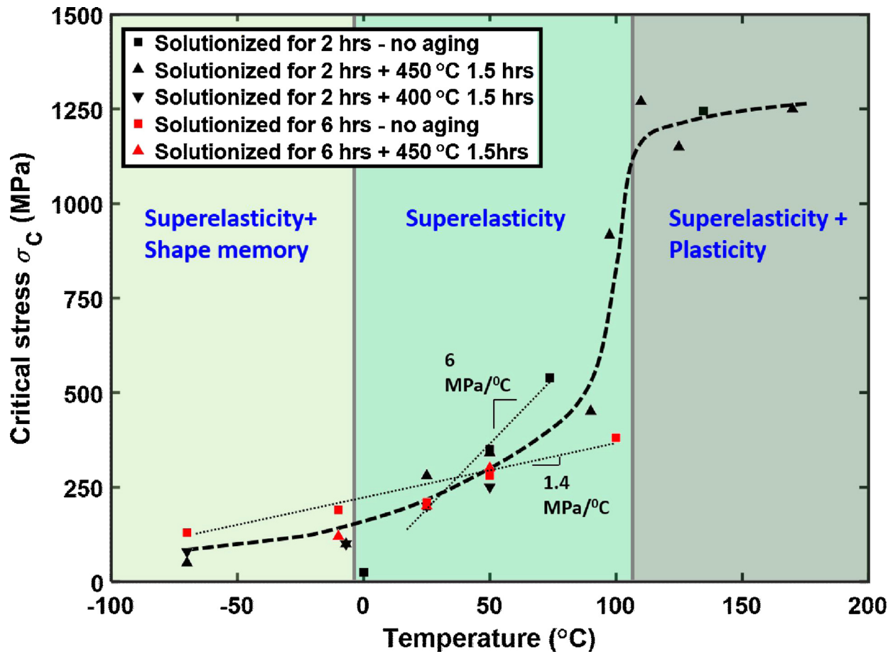
Fig. 3. Flow stresses as a function of temperature for \text{Ti}_{16.67}\text{Zr}_{16.67}\text{Hf}_{16.67}\text{Ni}_{25}\text{Co}_{10}\text{Cu}_{15} . The Clausius-Clapeyron slope is in the range of 1.4 MPa/°C for a lower bound and 6 MPa/°C for and upper bound and is indicated on the figure.
