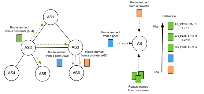
Figure 1: Examples of BGP export rules (left) and route preference (right). Green, blue, and orange rectangles represent routes learned from customer, peer, and provider, respectively.
