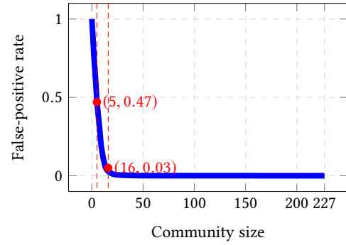
Figure 9: False-positive rate vs. community size.
