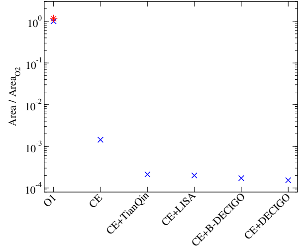
FIG. 8. Ratios of the areas of the 90% credible regions relative to that found with the LIGO O1 detector (Fisher result) shown in Fig. 7 for GW150914-like events, obtained from a Fisher analysis (blue cross). We report good agreement within 10% between the LIGO O1 Fisher and Bayesian [14] (red star) results. We also observe up to three orders of magnitude of improvement from the results of LIGO O1 to CE, and a further improvement of 7–10 times upon the use of multiband observations.
