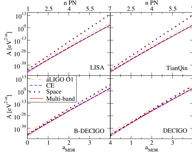
FIG. 11. 90% upper-bound constraints on the magnitude of the correction to the graviton dispersion relation \mathbb{A} as a function of a_{\text{MDR}} , found in Eq. (A11). Such bounds are computed from the ppE parameter for propagation mechanisms \beta_{\text{prop}} for GW150914-like events on various space- and ground-based detectors, and the combination of the two. Constraints on modifications to GR can be found by selecting a value of \alpha and mapping \mathbb{A} to its corresponding form, e.g., for massive gravitons with a_{\text{MDR}} = 0 and \mathbb{A} = m_g^2 , with bounds displayed in Table I and Fig. 5.
