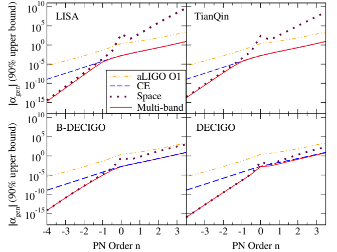
FIG. 9. Similar to Fig. 3, but for generation effects \alpha_{\text{gen}} entering the GW amplitude. Observe how for the case of amplitude corrections, multiband observations do not provide for much improvement over space-based detectors for negative-PN orders, and ground-based detectors for positive-PN orders.
