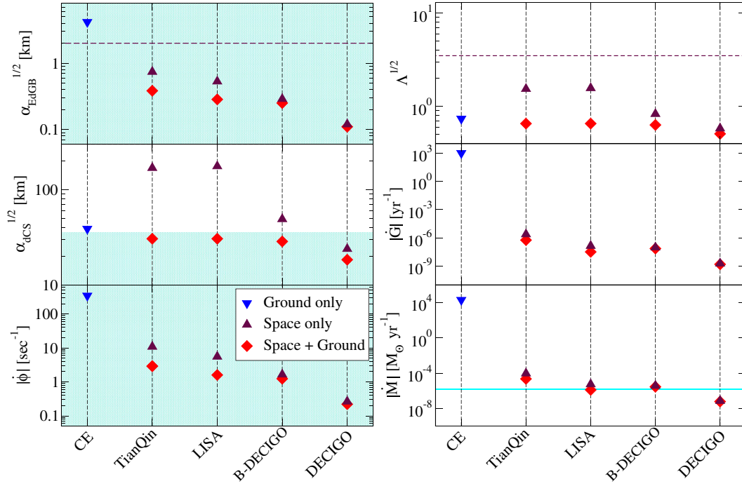
FIG. 4. 90% upper-bound credible level constraints on the theoretical parameters representative of six of the modified theories of gravity considered in this analysis for GW150914-like events. Bounds are presented for EdGB gravity ( \sqrt{\alpha_{\text{EdGB}}} , -1\text{PN} order), dCS gravity ( \sqrt{\alpha_{\text{dCS}}} , +2\text{PN} order), scalar tensor theories ( \dot{\phi} , -1\text{PN} order), noncommutative gravity ( \sqrt{\Lambda} , +2\text{PN} order), varying- G theories ( \dot{G} , -4\text{PN} order), and BH mass-varying theories ( \dot{M} , -4\text{PN} order), and are additionally tabulated in Table I. The blue shaded regions correspond to the region such that the small coupling approximations \zeta_{\text{EdGB}} \ll 1 , \zeta_{\text{dCS}} \ll 1 , and m\dot{\phi} \ll 1 are valid (the definition of the dimensionless coupling constants \zeta can be found in Appendix A), and the dashed maroon lines correspond to the current bounds in the literature, also tabulated in Table I. The cyan line in the bottom right panel corresponds to the Eddington accretion rate for GW150914-like events.
