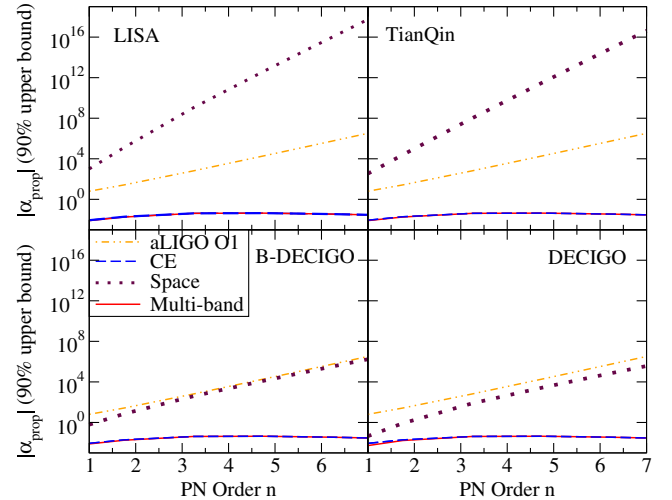
FIG. 10. Similar to Fig. 3, but for propagation effects \alpha_{\text{prop}} entering the GW amplitude. Observe how for the case of amplitude corrections, multiband observations do not provide for much improvement over the constraints provided by CE.
