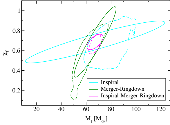
FIG. 7. 90% credible region contours of the inspiral, merger-ringdown, and complete waveform posterior distributions in the M_f - \chi_f plane, for GW150914-like events observed on the LIGO O1 detector. We present both the Fisher analysis results (solid) discussed here and the Bayesian results of Ref. [14] (dashed) for comparison. We observe good agreement between the two analyses in both the direction of correlation, and in the overall areas, which agree to within 10% for all three distributions.
