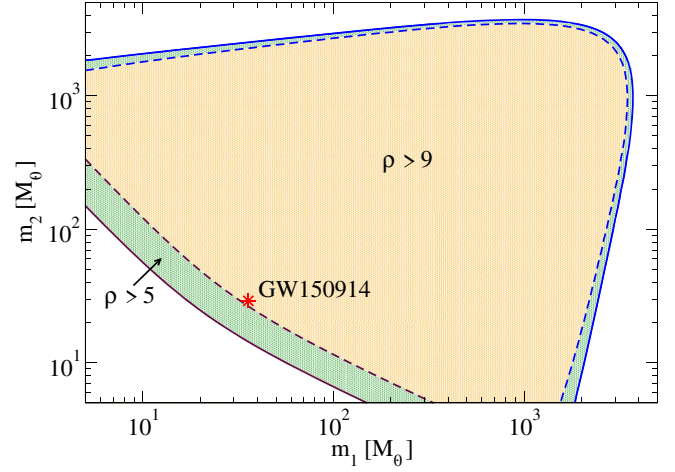
FIG. 2. Multiband detectability region as a function of the constituent BH masses m_1 and m_2 . This region is formed by SNRs in agreement with the condition \rho > \rho_{\text{th}} for \rho_{\text{th}} = 5 (optimistic) and \rho_{\text{th}} > 9 [39,40] (pessimistic) for events detected by both the ground-based detector CE, and space-based detector LISA. Such SNRs have been computed with the assumption of nonspinning BHs at luminosity distances of 410 Mpc. The upper-right edge (blue) of the region corresponds to CE's \rho_{\text{th}} contour, while the lower-left edge (maroon) is formed by LISA's contour. The SNRs are computed following Eq. (3). Additionally shown as a red star is the event GW150914 with (m_1, m_2) = (35.8 M_\odot, 29.1 M_\odot) . Observe how GW150914-like events marginally fall within LISA's larger observational SNR threshold of \rho_{\text{th}} = 9 . Alternatively, such events exceed both ground-based SNR thresholds by more than 2 orders of magnitude.
