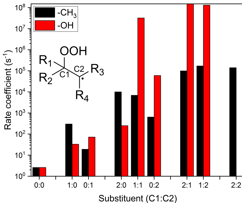
Figure 2: Reaction rate coefficient for epoxide formation in the systems with zero to four methyl or hydroxy substituents at R_1 to R_4 . The remaining substituents are hydrogens. The systems are denoted by the number of methyl or hydroxy substituents at C1 and C2 as C1:C2. For the system with four OH substituents, the transition state geometry optimization would not converge.
