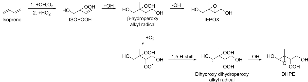
Scheme 1: Reaction mechanism leading from isoprene to one isomer of IEPOX and the isoprene dihydroxy hydroperoxy epoxide (IDHPE) proposed by D'Ambro et al. 12
