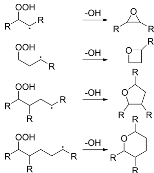
Figure 5: Illustration of formation of an epoxide (3-membered ring) along with formation of 4-, 5- and 6-membered cyclic ethers. Different systems with one or more substituents at positions R were studied (see Figure S8).
