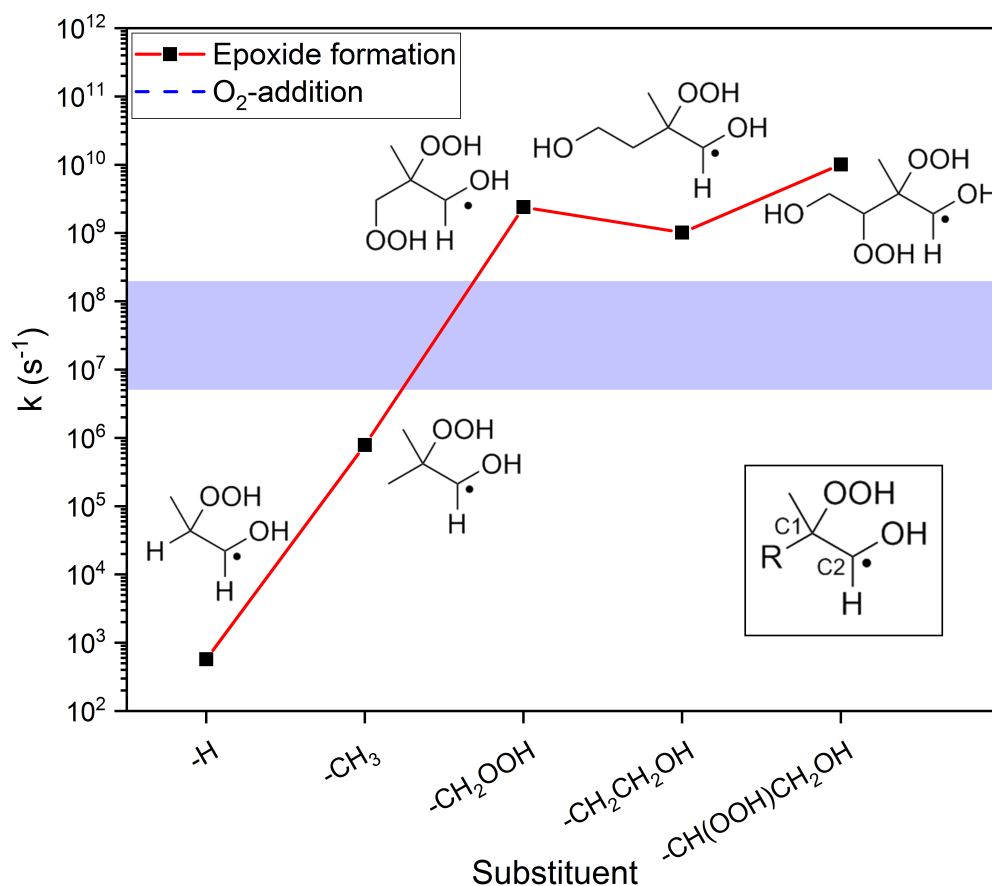
Figure 4: Reaction rate coefficient of epoxide formation as a function of the substituent at position R (C1) in the insert. The shaded blue region represents the pseudo first-order rate coefficient of O 2 -addition in the range 5 \times 10^6 \text{ s}^{-1} - 2 \times 10^8 \text{ s}^{-1} (see text).
