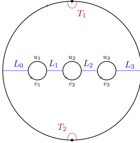
FIGURE 6. Sphere with 4 holes, 2 stops, a generating set of Lagrangians ( L_i ) and certain other Lagrangians supported near stops ( T_1 and T_2 )
