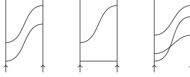
FIGURE 3. A strand diagram with 3 boundary components
