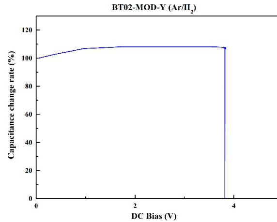
Figure 10. Capacitance change with DC bias for BT02-MOD-Y.
