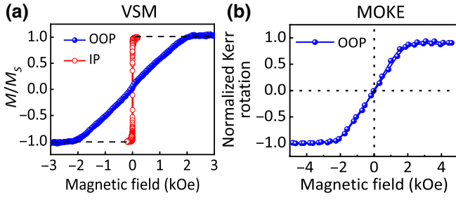
FIG. 3. Magnetic hysteresis responses of a 6-nm-thick YIG film grown on a GGG substrate. (a) VSM data measured under an OOP field and an IP field. (b) Polar MOKE data measured under an OOP field.
