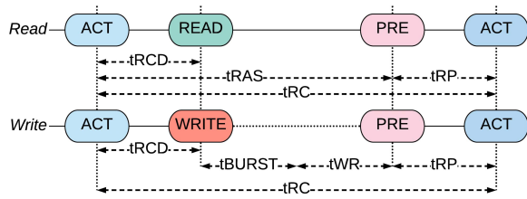
Figure 4. PCM timings for serving read and write requests.
