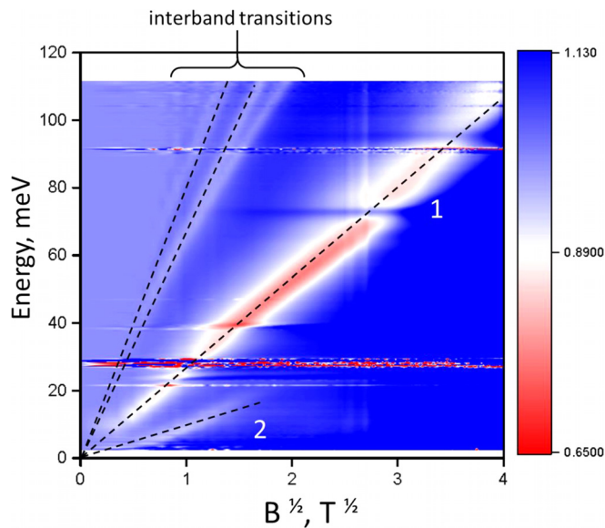
FIG. 2. Color plot of the absorption as a function of the emission energy and square root of the magnetic field. Line 1 corresponds to the transition between the 0th and the 1st electron Landau level and line 2 to the transition between the 1st and the 2nd electron Landau level. The dashed lines are guides to the eye.
