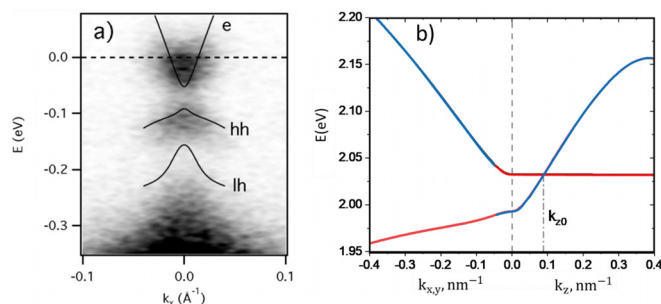
FIG. 3. (a) ARPES spectrum of the InAsSb/InSb SL with a period of 7.8 nm, recorded at T = 108 K. The solid lines represent the 8-band k \cdot p calculations. (b) Calculated carrier dispersion of the band-inverted SL for k_{x,y} and k_z . The blue curve indicates electronlike states, while the red curve indicates the holelike ones.
