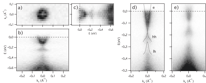
FIG. 1. The electronic structure of InAs 0.48 Sb 0.52 /InSb SL with a period of 6.2 nm. The Fermi surface (a) and dispersion of the low-energy excitations along the two perpendicular momentum lines [(b) and (c)] indicate an isotropic in-plane electronic structure. The low-temperature electronic structure [(a)–(d)] is nearly gapless. The 300 K spectrum (e) shows a finite gap. Dashed lines in (d) are band-fits based on 8 \times 8 k \cdot p calculations. 18
