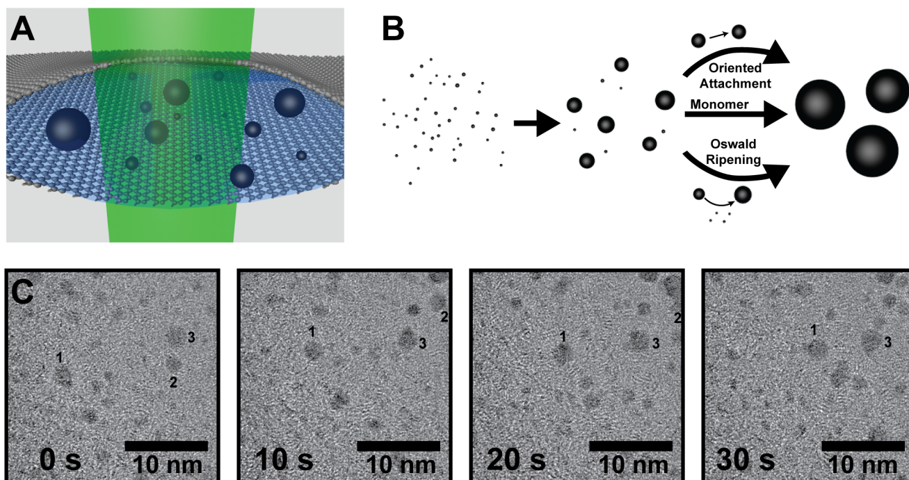
Figure 4. Using graphene liquid cell electron microscopy to observe platinum nanocrystal growth. (A) Schematic of nanocrystals (black) encapsulated in solution between two graphene sheets while imaging with the electron beam (green beam). (B) Schematic showing examples of the pathways of growth for nanocrystals from a solution of monomer platinum atoms. The examples shown are attachment, monomer addition, and Ostwald ripening. (C) Example images from the electron microscopy video of platinum nanocrystal growth. Nanocrystals can be seen moving and growing in size. Three example nanoparticles are labeled.
