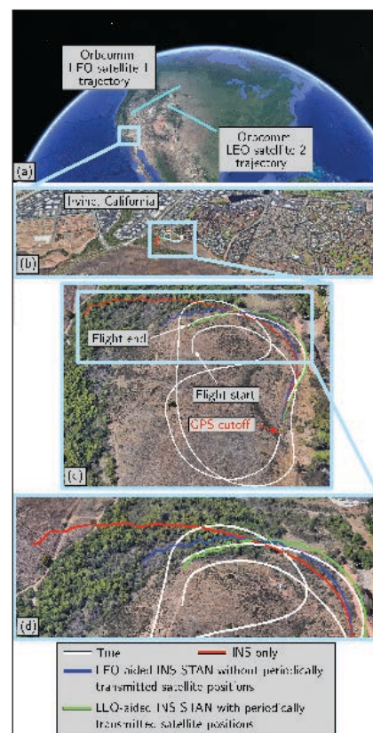
FIGURE 24 Results of the UAV experiment. (a) Orbcomm satellite trajectories. (b)-(d) UAV's true and estimated trajectories. Map data: Google Earth.
