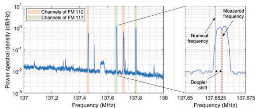
FIGURE 17 Snapshot of the Orbcomm spectrum.
