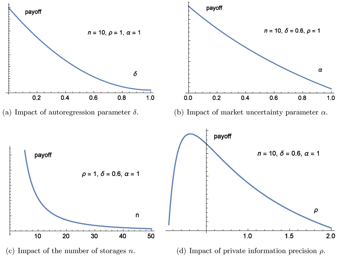
Fig. 2. Sensitivity analysis of individual storage's payoff with respect to model primitives.
