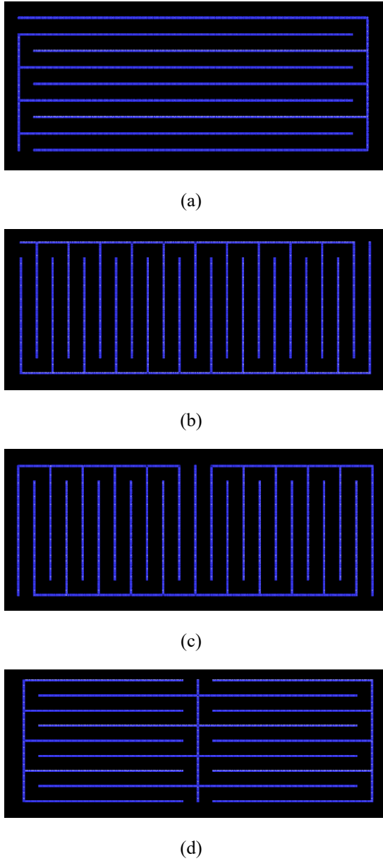
Figure 9. Rectangular winding queue layouts: (a) Config.1, (b) Config.2, (c) Config.3, (d) Config.4.
