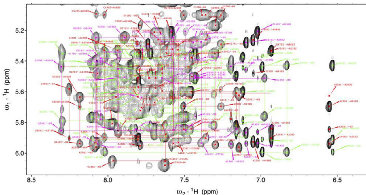
Fig. 7. Typical H1'-H6/H8 assignment 'walk' for an RNA thermometer Spectral assignments were confirmed using the smaller constructs of Fig. 5 which are shown with various colored lines. (For interpretation of the references to colour in this figure legend, the reader is referred to the web version of this article.)
