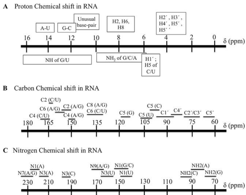
Fig. 6. Chemical shifts for nuclei in RNA from the BMRB data bank
