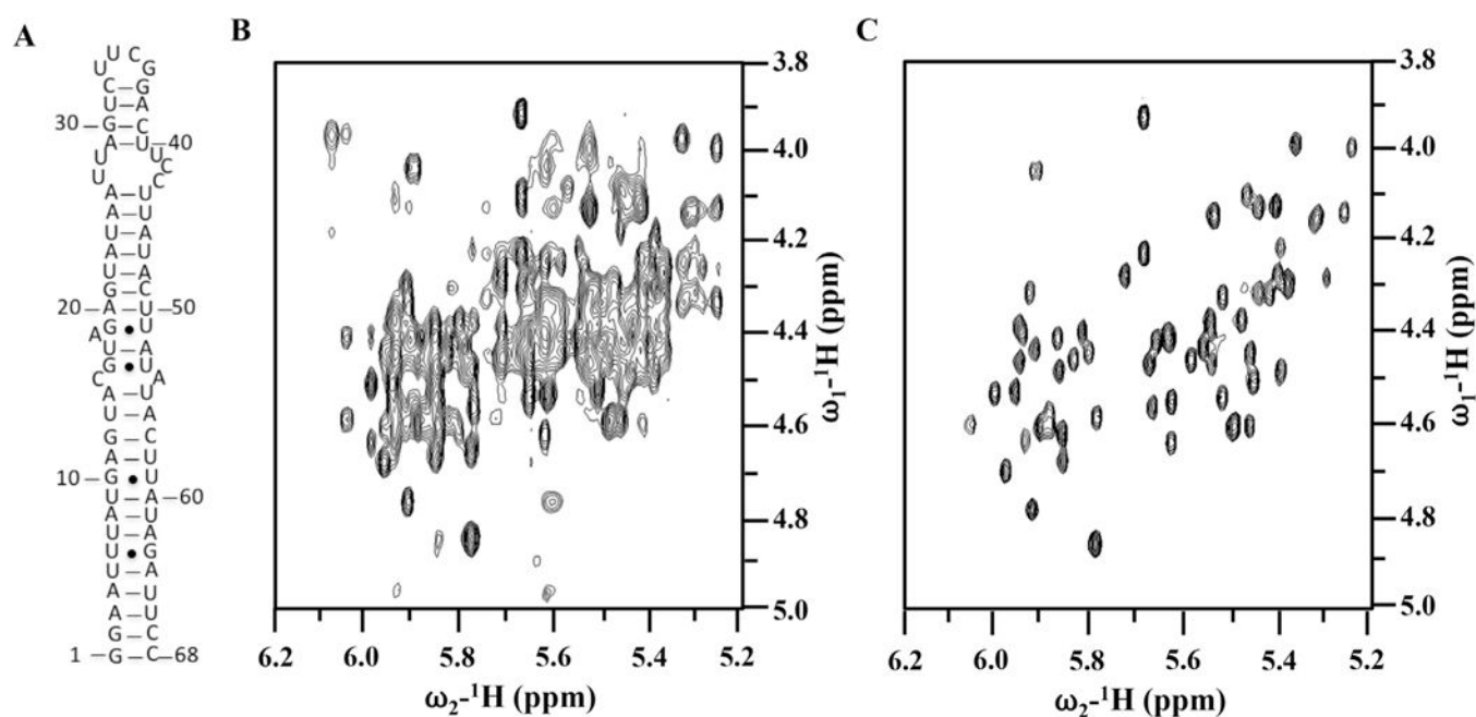
Fig. 4. Effect of site-specific ribose deuteration on the quality of the NMR spectra of an RNA thermometer
