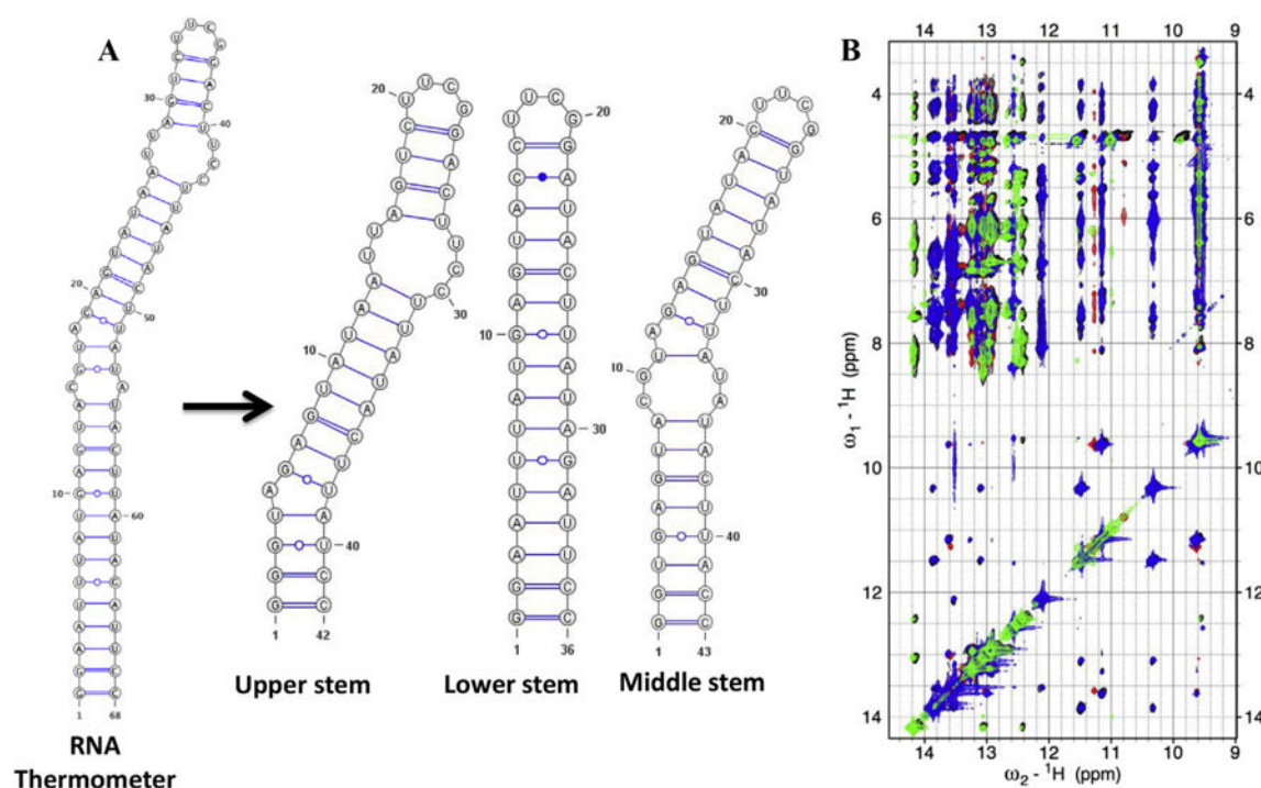
Fig. 3. NMR Assignment strategy for an RNA thermometer of ~70 nucleotides
