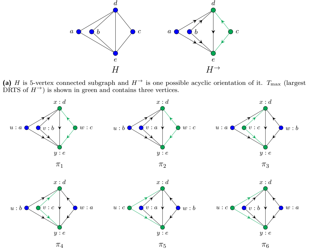
(b) All six figures show exactly the same subgraph in G^\rightarrow . \pi_1, \dots, \pi_6 are six equivalent matches of H^\rightarrow in G^\rightarrow , one for each automorphism of H^\rightarrow . Notice (u, v, w) being mapped to all permutations of (a, b, c) .
