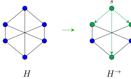
Figure 5 Alg. 2 succeeds to count the number of distinct matches of H in linear time for bounded (constant) degeneracy graphs. Each acyclic orientation of H has a source vertex s , which is connected to exactly three vertices, as in H^\rightarrow . So, the largest DRTS has at least four vertices (shown in green). Number of matches of the remaining vertices (shown in blue) could be counted using \mathcal{HM}_2 .
