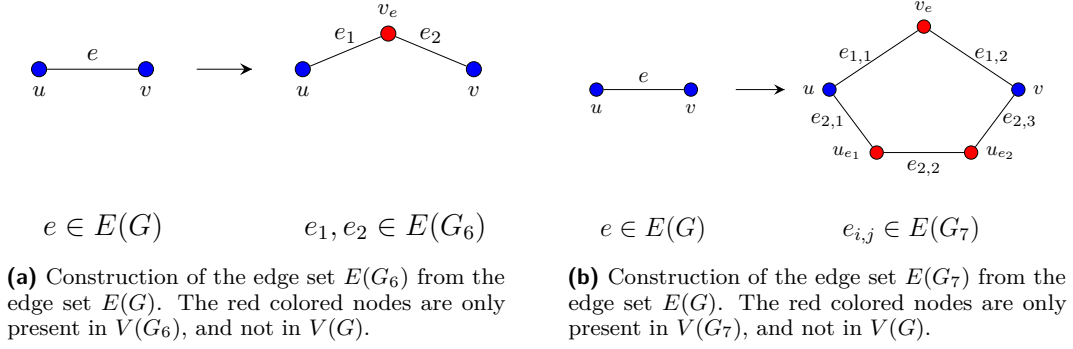
■ Figure 4 Reduction from the TRI-CNT problem to the SUB-CNT k problem for k = 6 (left) and k = 7 (right).
