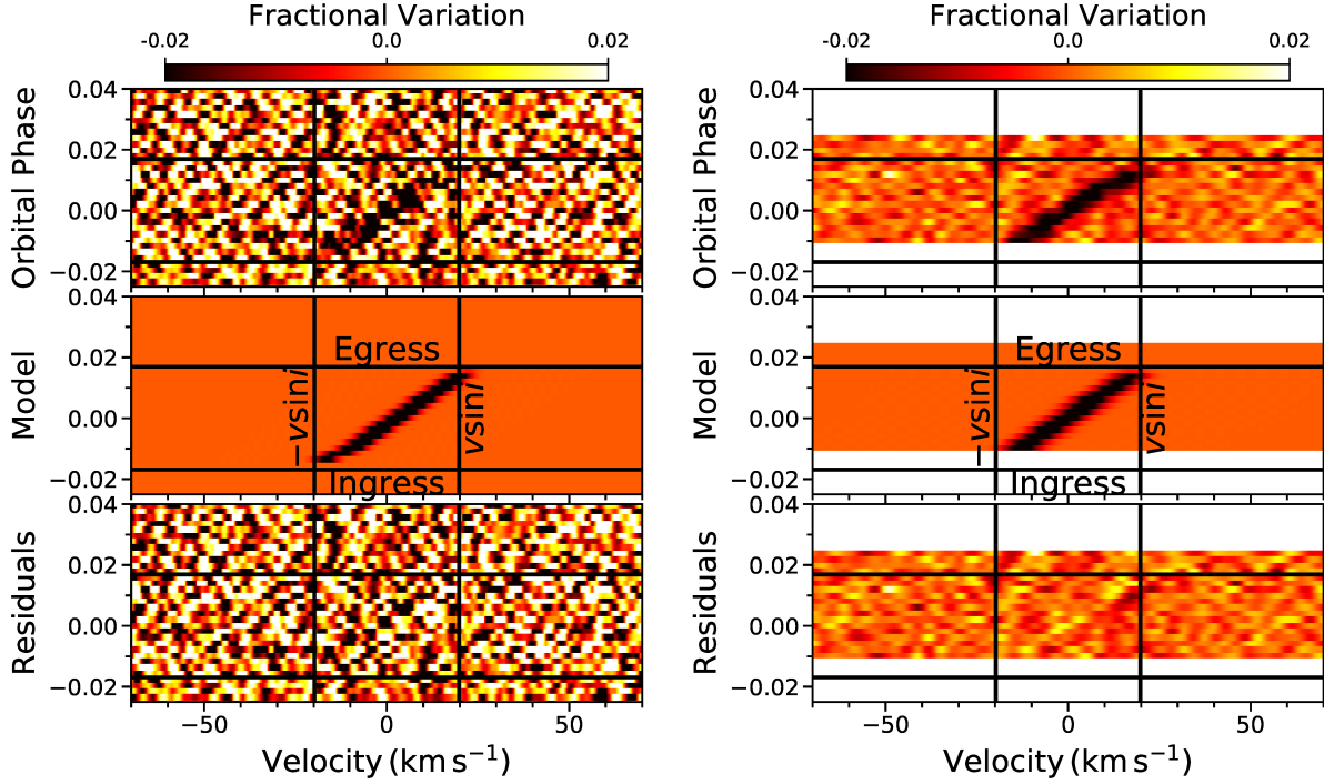
Figure 4. The Doppler Tomographic transit of KELT-24 b on UT 2018 March 31 from (Left) MINERVA and (Right) TRES. The overall average of the line profiles from each instrument are plotted as a function of orbital phase and velocity. The MINERVA observation is the combined Doppler tomographic signal from telescopes 2 and 3 (see §2.4). The top panel in each plot represents the observed transit. The middle and bottom panels show the best-fit models and residuals after the model has been subtracted. MINERVA observed the entire transit, with baseline on each side, while TRES did not observe the beginning of the transit.
